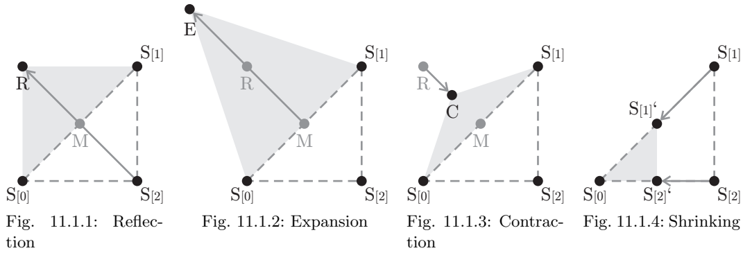
Fig. 11.1: One possible step of the downhill simplex algorithm applied to a problem in \mathbb{R}^2 .
