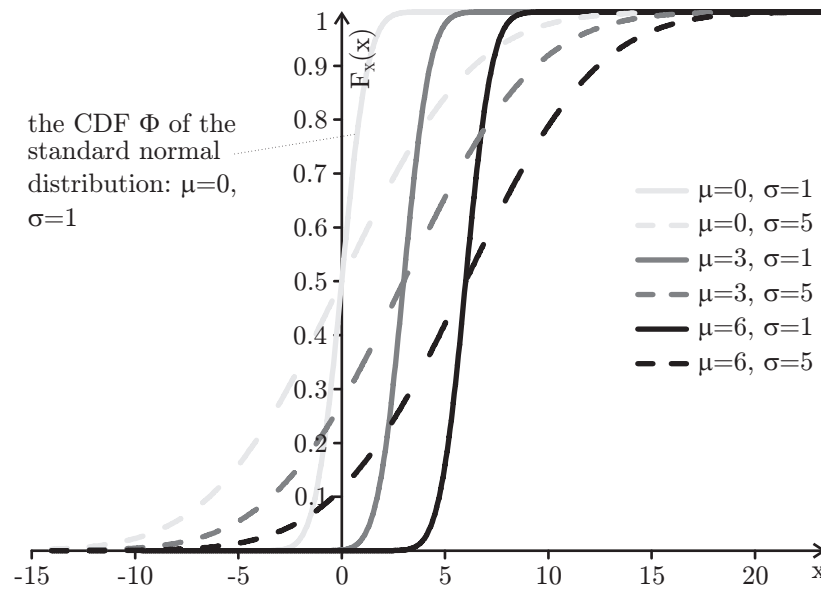
Fig. 27.10: The CDFs of some normal distributions
