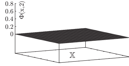
Fig. 1.17.2: \Phi(x, 2)
