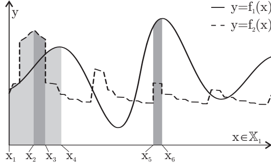
Fig. 1.8: Optimization using the Pareto Frontier approach.
