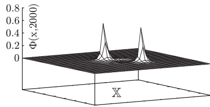
Fig. 1.17.9: \Phi(x, 2000)
