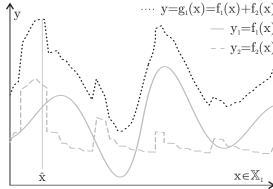
Fig. 1.5: Optimization using the weighted sum approach (first example).
