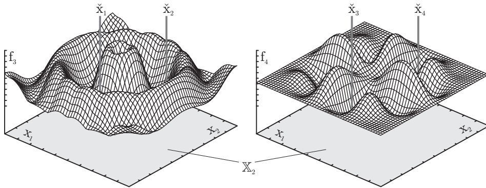
Fig. 1.4: Two functions f_3 and f_4 with different minima \check{\mathbf{x}}_1 , \check{\mathbf{x}}_2 , \check{\mathbf{x}}_3 , and \check{\mathbf{x}}_4 .
