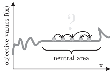
Fig. 1.20.6: Neutral
