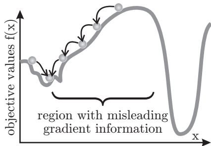
Fig. 1.20.5: Deceptive
