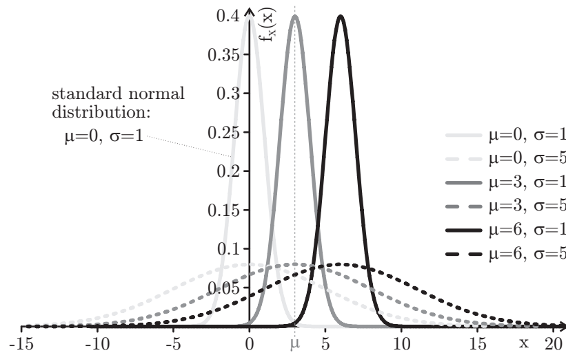
Fig. 27.9: The PDFs of some normal distributions
