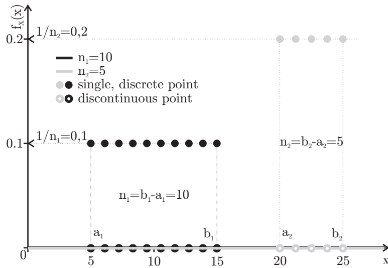
Fig. 27.1: The PMFs of some discrete uniform distributions
