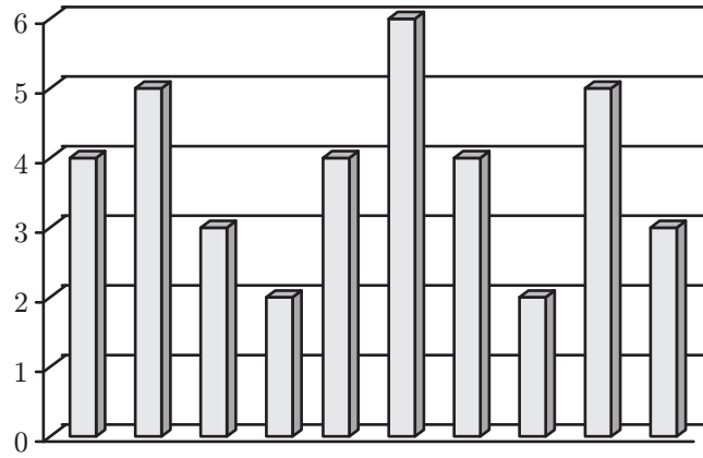
Fig. 27.18: The numbers thrown in the dice example
