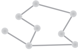
Fig. 29.3.1: unrestricted topology
