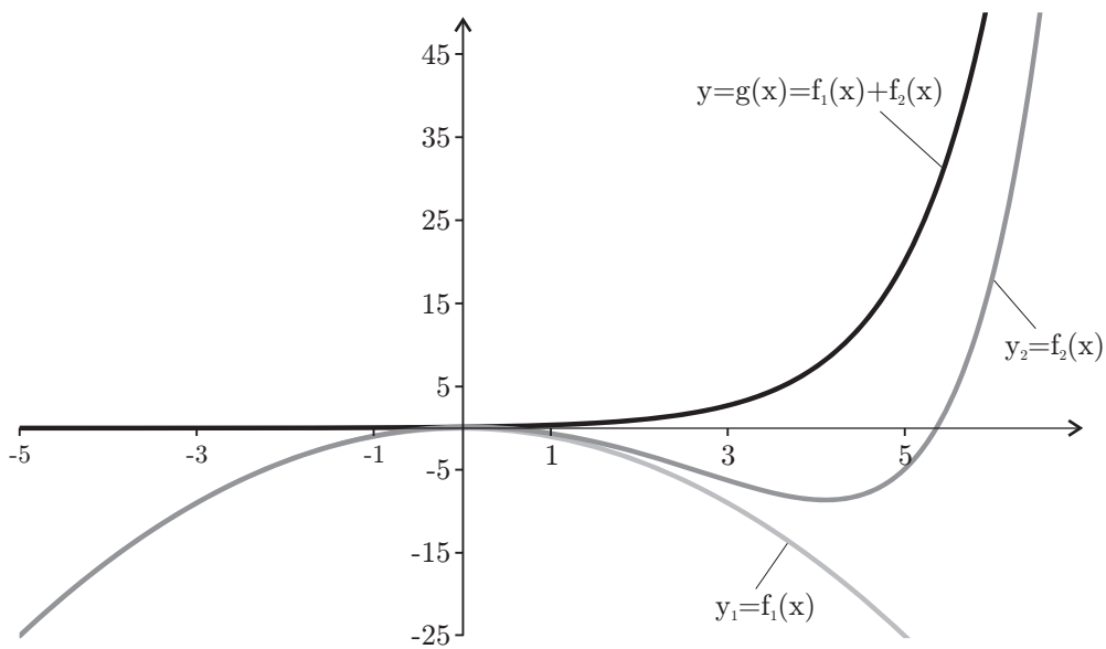
Fig. 1.7: A problematic constellation for the weighted sum approach.
