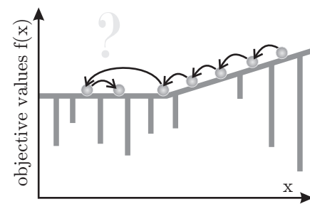
Fig. 1.20.8: Nightmare
