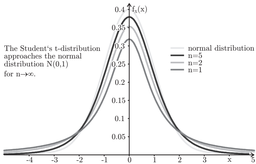
Fig. 27.15: The PDFs of some Student's t-distributions
