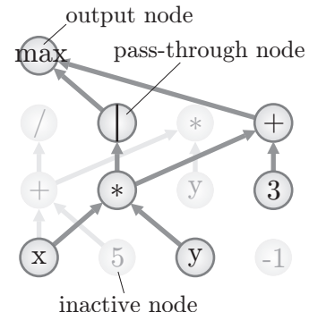
Fig. 4.23.3: PDGP structure
