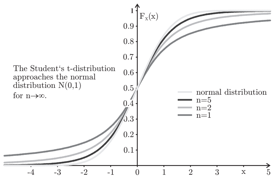
Fig. 27.16: The CDFs of some Student's t-distributions
