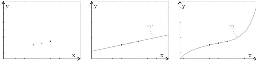
Fig. 1.23.1: Three sample points of f_1 .
