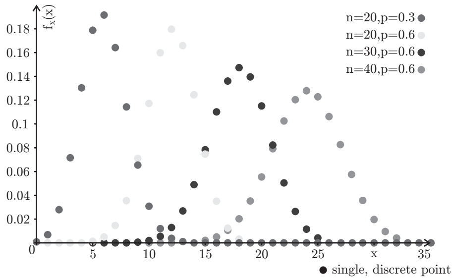
Fig. 27.5: The PMFs of some binomial distributions
