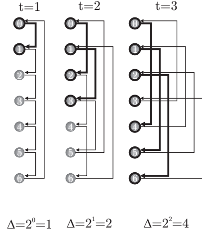
Fig. 23.14.2: general
