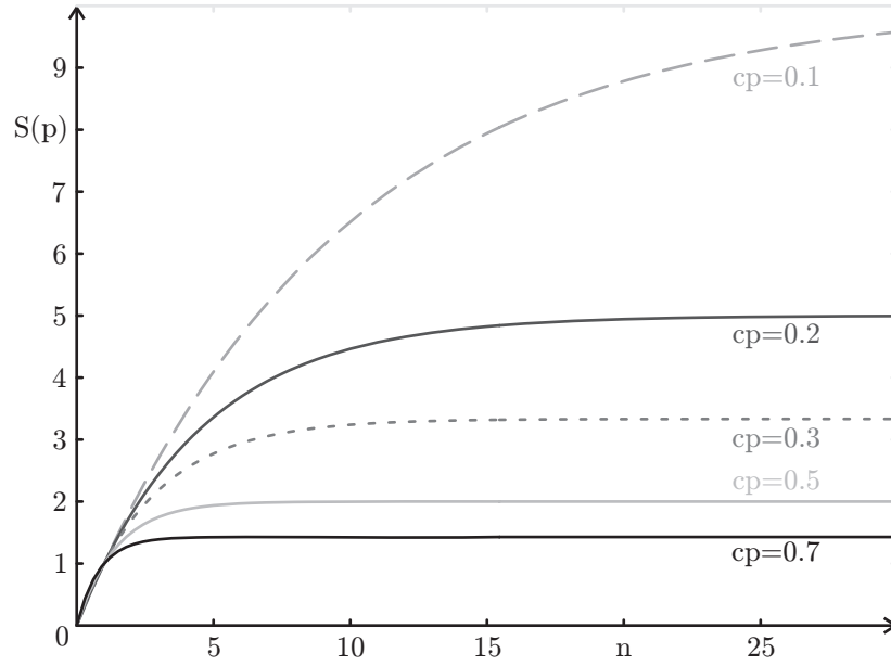
Fig. 2.12: The expected numbers of occurrences for different values of n and cp .
