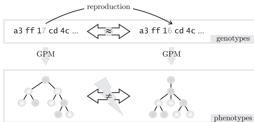
Fig. 4.26: Epistasis in a Grammatical Evolution-like approach.
