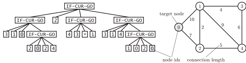
Fig. 23.4: An evolved routing rule set (left) with target node 0 for the specified network (right).
