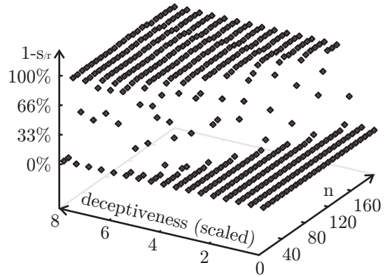
Fig. 20.9.4: Scaled deceptiveness – failed runs
