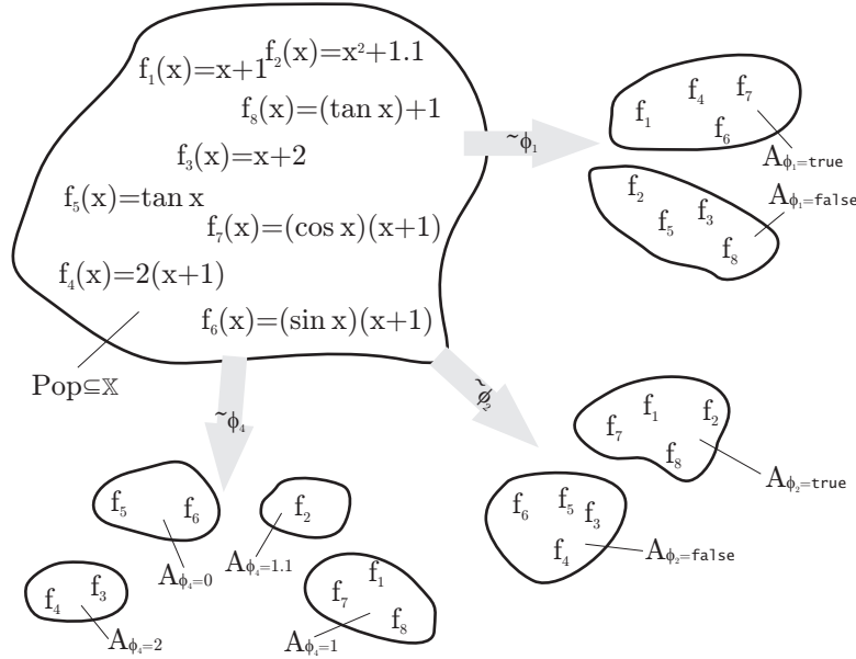
Fig. 1.29: Example for formae in symbolic regression.
