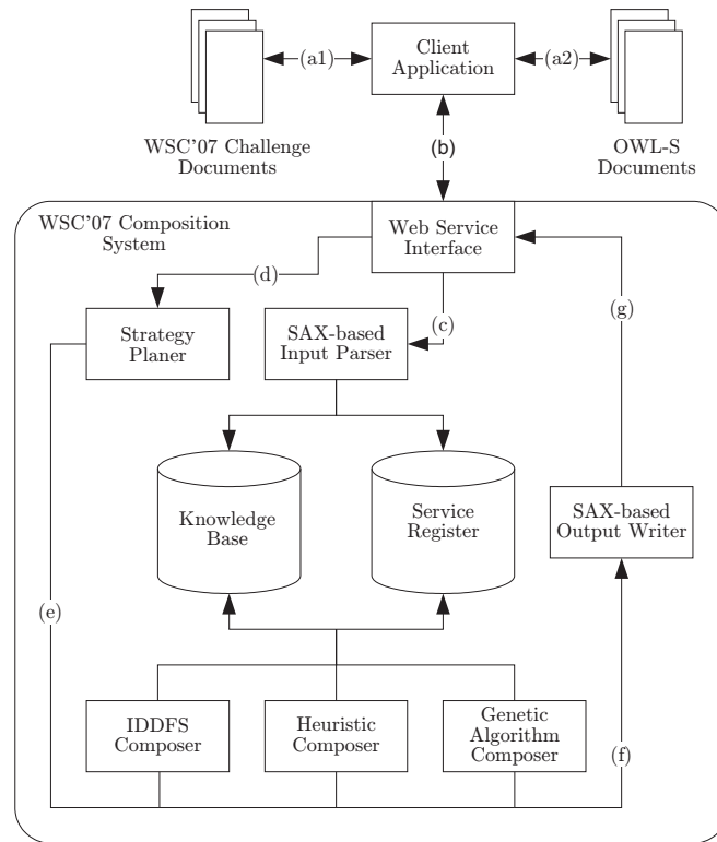
Fig. 21.10: The WSC 2007 Composition System of Bleul et al. [1604; 1605].
