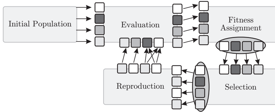
Fig. 17.1: Parallelization potential in evolutionary algorithm.
