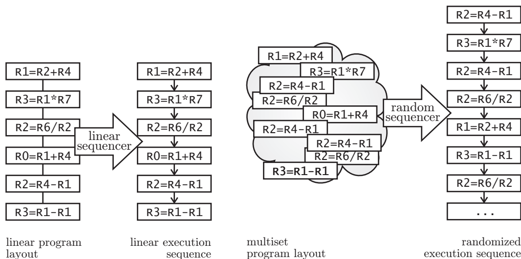
Fig. 4.28.1: Linear Genetic Programming phenotype and execution.
