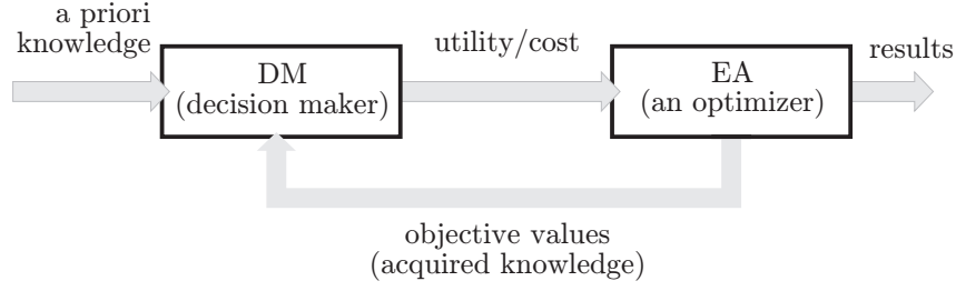
Fig. 1.12: An external decision maker providing an evolutionary algorithm with utility values.
