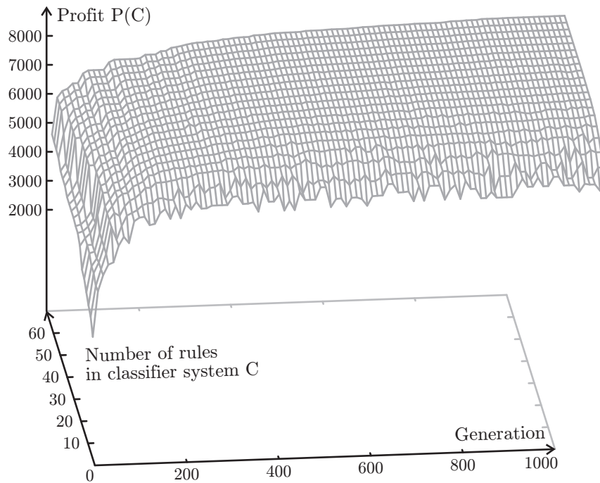
Fig. 21.7: The course of the modified classifier system evolution.
