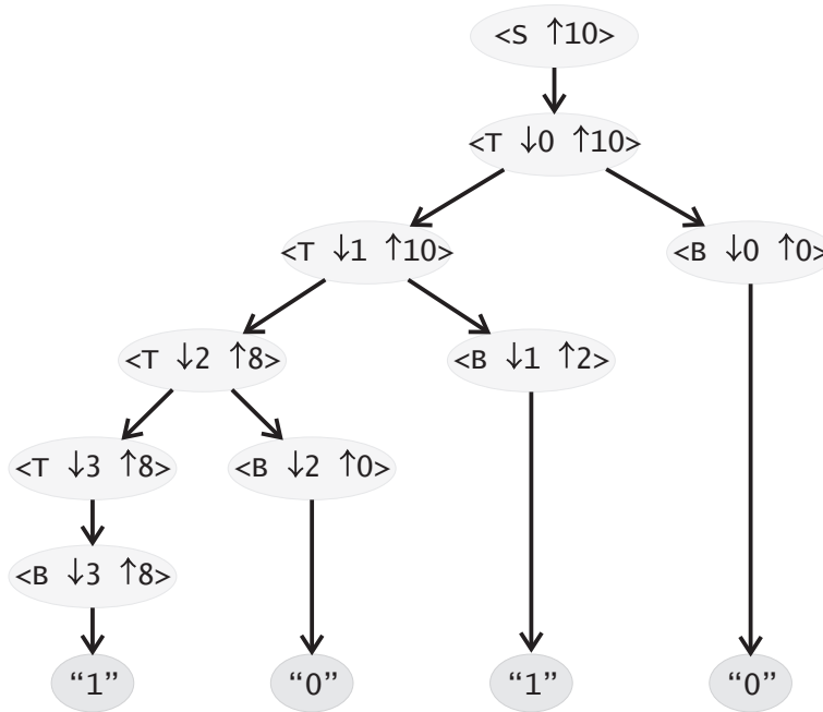
Fig. 29.14: One possible expansion of the example grammar G_2 .
