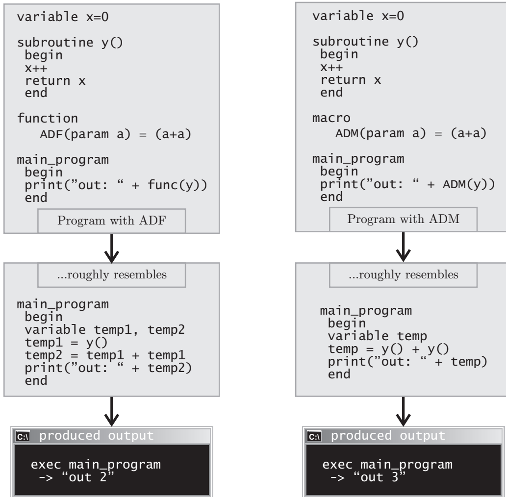
Fig. 4.13: Comparison of functions and macros.
