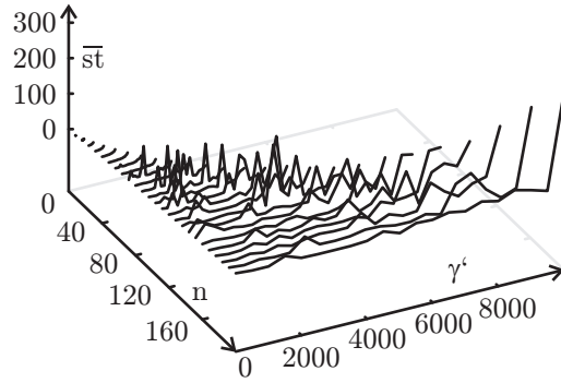
Fig. 20.9.1: Unscaled ruggedness \bar{st} plot.
