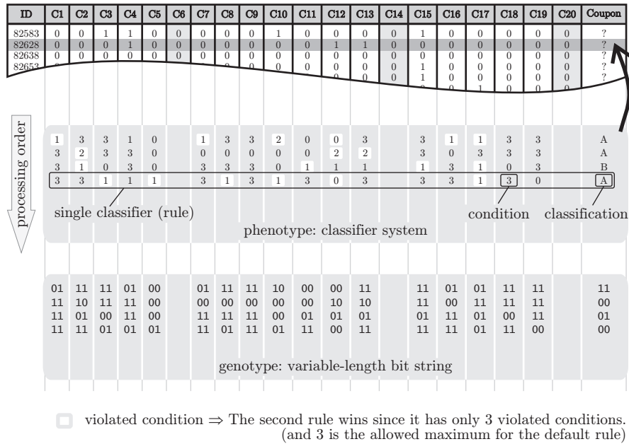
Fig. 21.4: An example classifier for the 2007 DMC.
