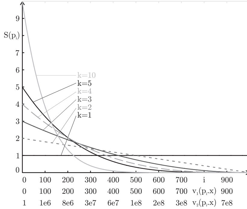
Fig. 2.10: The number of expected offspring in tournament selection.
