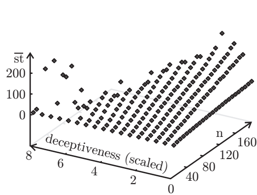
Fig. 20.9.3: Scaled deceptiveness – average success generations \bar{st}
