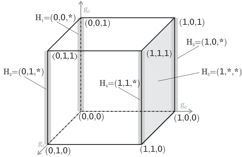
Fig. 3.8: An example for schemata in a three bit genome.
