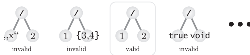
Fig. 4.17: Example for valid and invalid trees in typed Genetic Programming.
