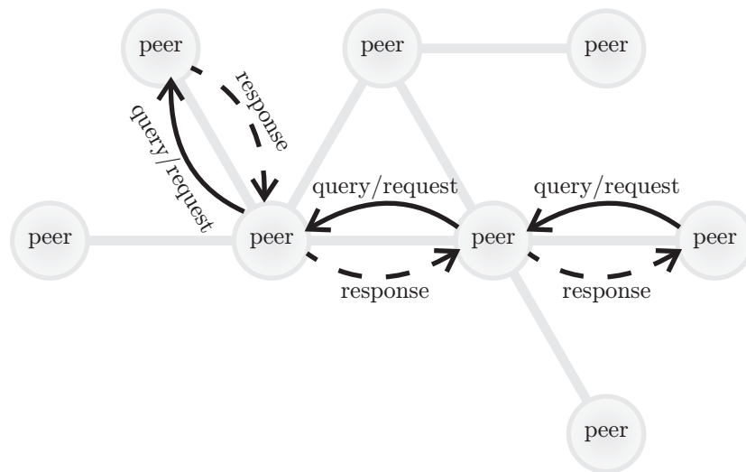
Fig. 29.5: A peer-to-peer system in an unstructured network
