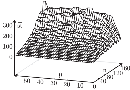
Fig. 20.11: The results from experiments with neutrality.
