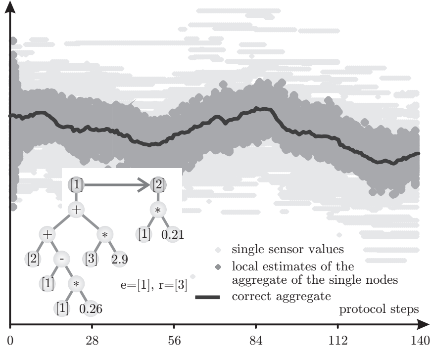
Fig. 23.17: A dynamic aggregation protocol for the distributed average.
