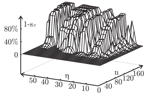
Fig. 20.10.2: Epistasis \eta and problem length n : failed runs.
