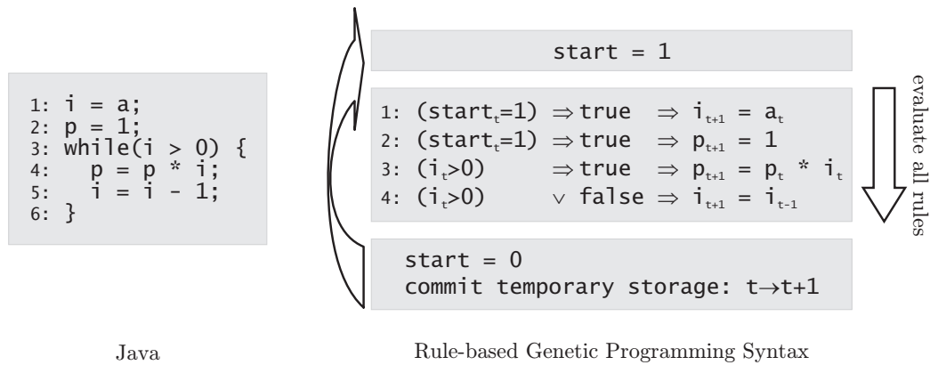
Fig. 4.30: A program computing the faculty of a natural number in Java and RBGP syntax.
