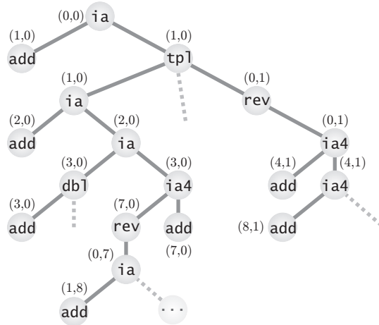
Fig. 23.3.4: The node-pair encoding GP (NP2).
