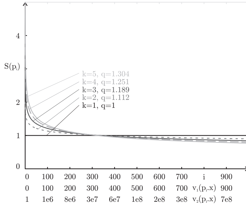
Fig. 2.11: The number of expected offspring in ordered selection.
