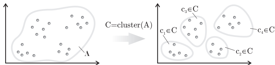
Fig. 28.1: A clustering algorithm applied to a two-dimensional dataset A .
