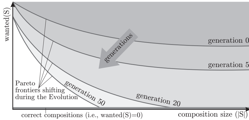
Fig. 21.9: A sketch of the Pareto front in the genetic composition algorithm.
