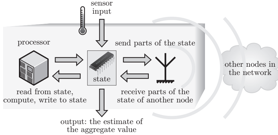
Fig. 23.15: The model of a node capable to execute a proactive aggregation protocol.
