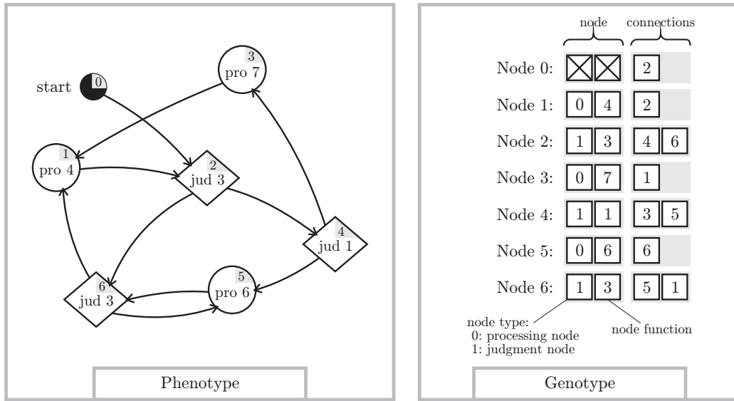
Fig. 4.24: An example program in Genetic Network Programming syntax.
