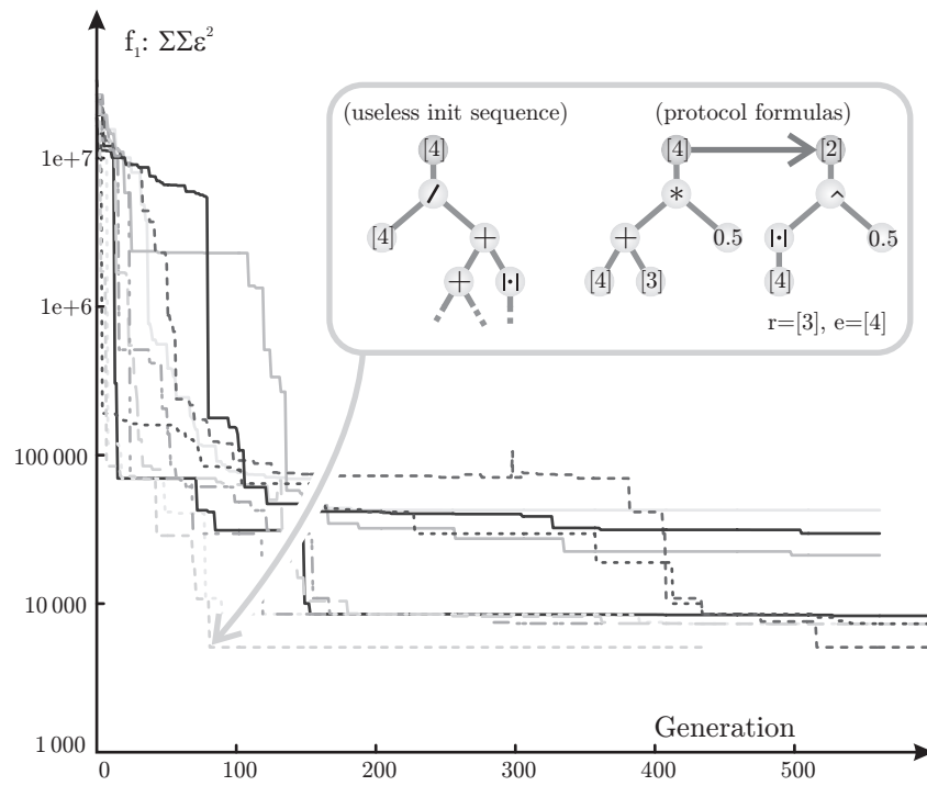
Fig. 23.21: The evolutionary progress and one grown solution of the static root-of-average protocol.
