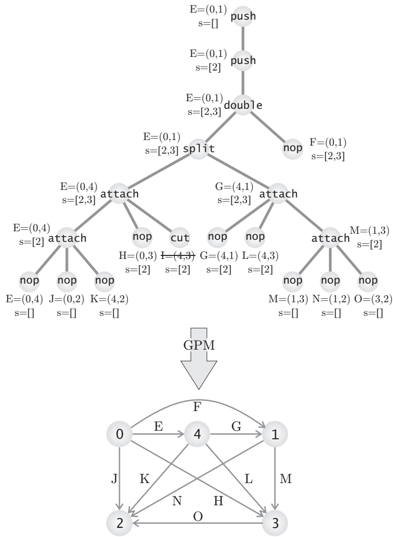
Fig. 4.15: An example for edge encoding.
