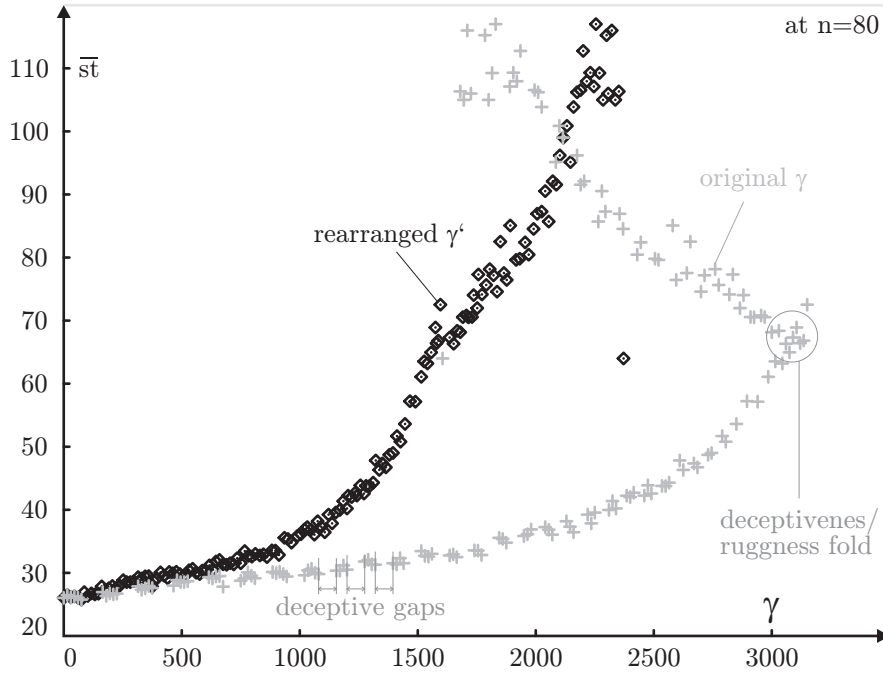
Fig. 20.8: Experimental results for the ruggedness.
