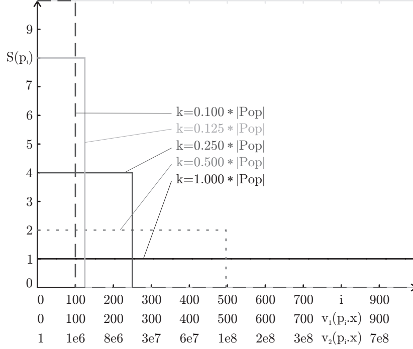
Fig. 2.7: The number of expected offspring in truncation selection.
