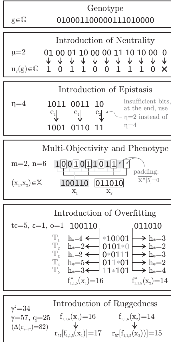
Fig. 20.4: An example for the fitness landscape model.
