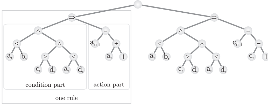
Fig. 4.31: The tree phenotype (and genotype) of Listing 4.15.
