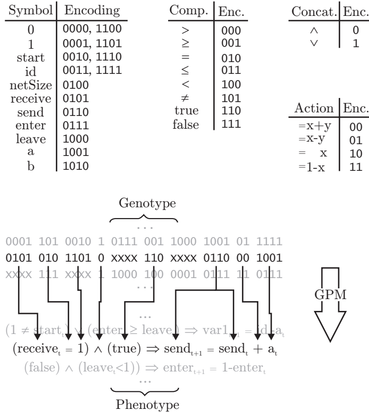
Fig. 4.29: genotype-phenotype mapping in Rule-based Genetic Programming.
