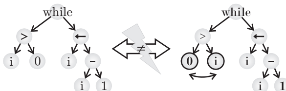
Fig. 4.27.2: In Standard Genetic Programming
