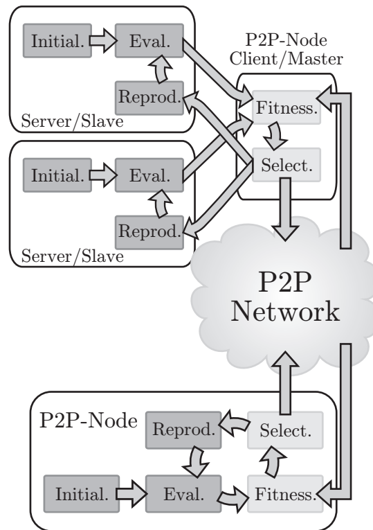
Fig. 17.7: A mixed distributed evolutionary algorithms.
