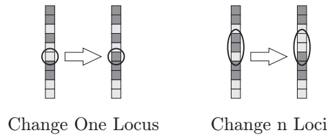
Fig. 3.3: Value-altering mutation of string chromosomes.
