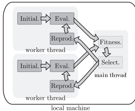
Fig. 17.3: A parallel evolutionary algorithm with two worker threads.
