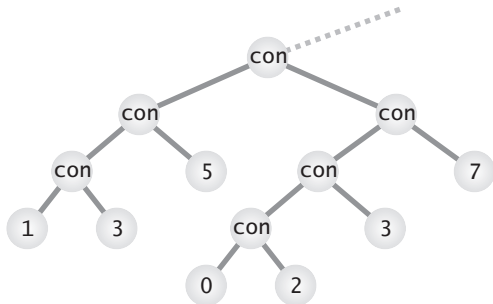
Fig. 23.3.3: The connective approach (CN).
