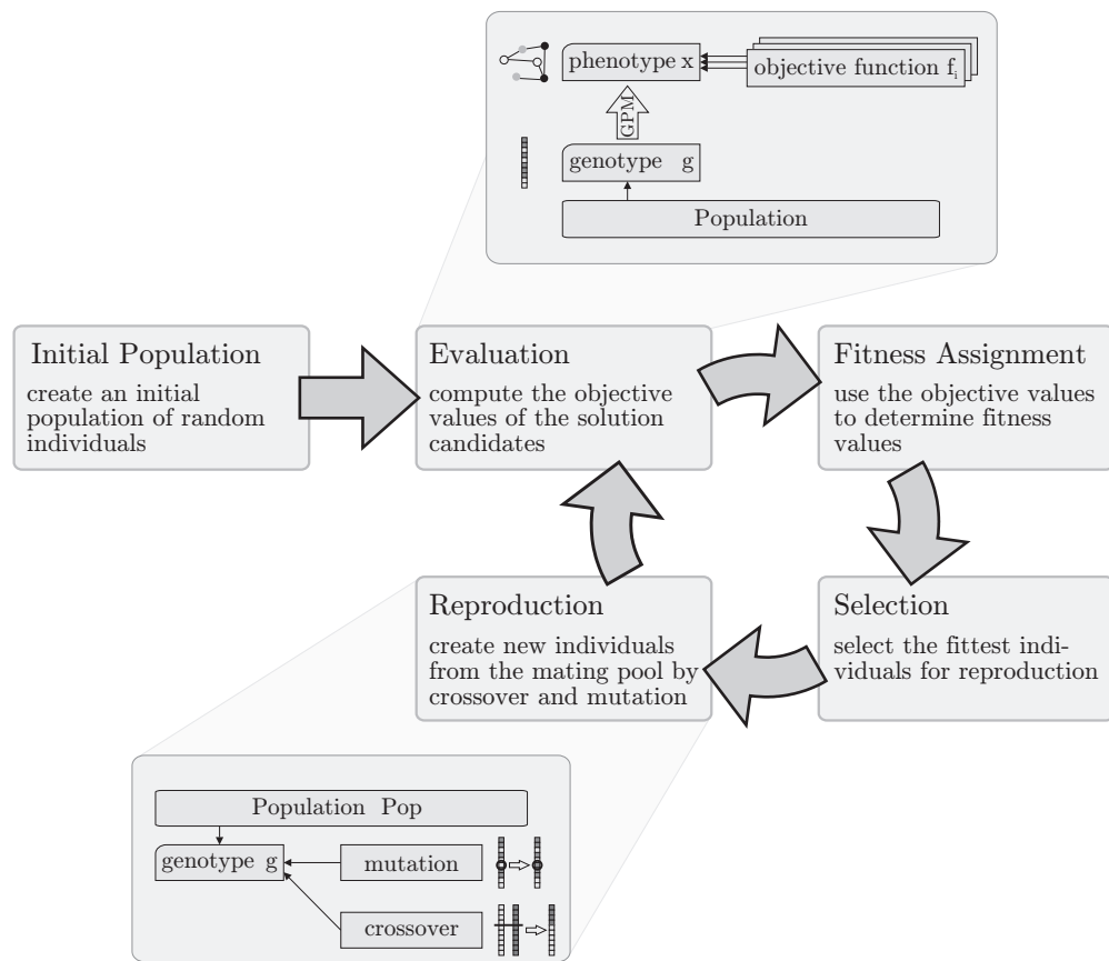
Fig. 3.1: The basic cycle of genetic algorithms.
