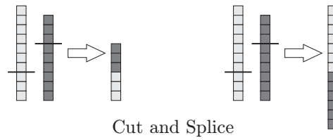
Fig. 3.7: Crossover of variable-length string chromosomes.
