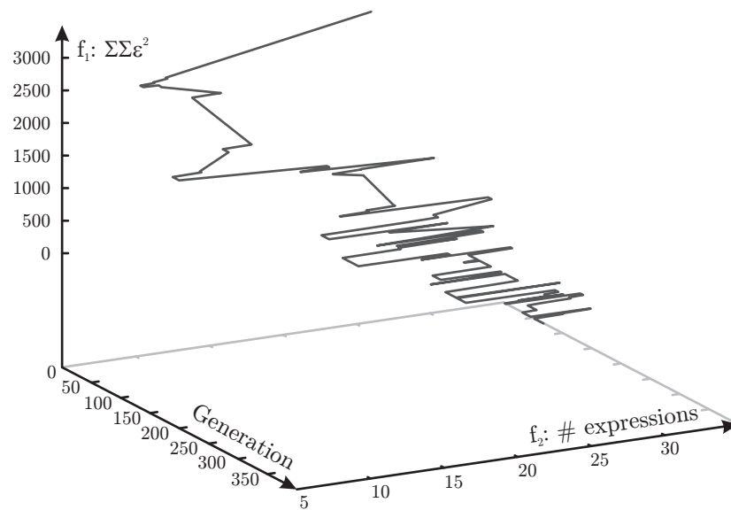
Fig. 23.24: The relation of f_1 and f_2 in the dynamic average protocol.
