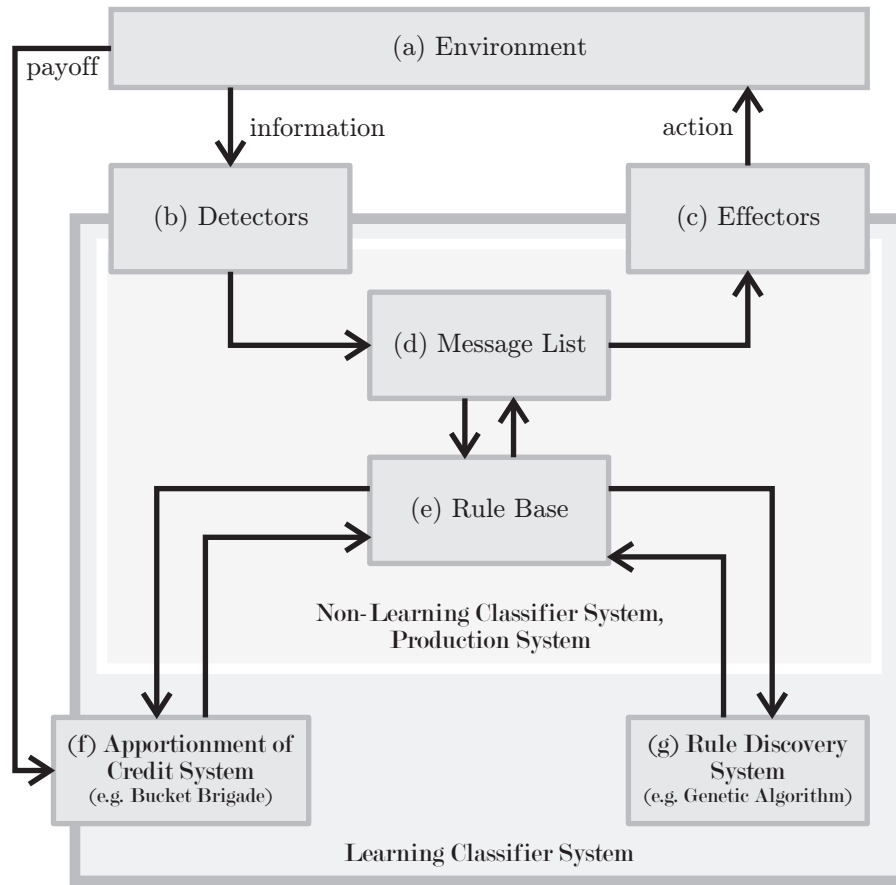
Fig. 7.1: The structure of a Michigan style Learning Classifier System according to Geyer-Schulz [1225].
