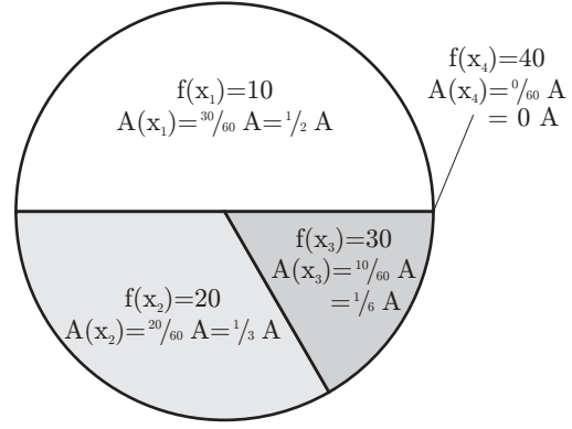
Fig. 2.8.2: Example for normalized fitness minimization.
