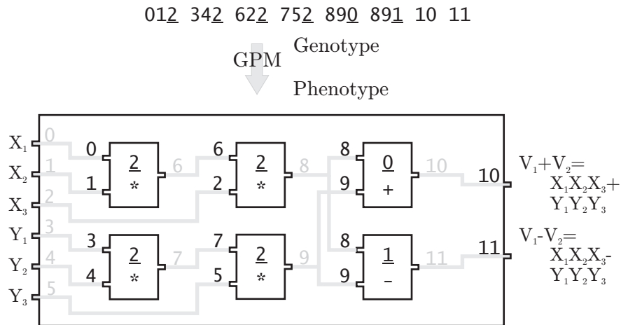
Fig. 4.25: An example for the GPM in Cartesian Genetic Programming.
