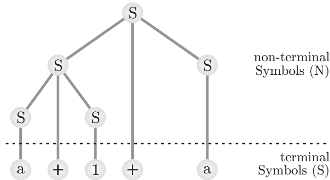
Fig. 29.12: The derivation of the example expansion of the grammar G .
