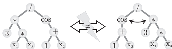
Fig. 4.27.1: In Standard Genetic Programming and symbolic regression
