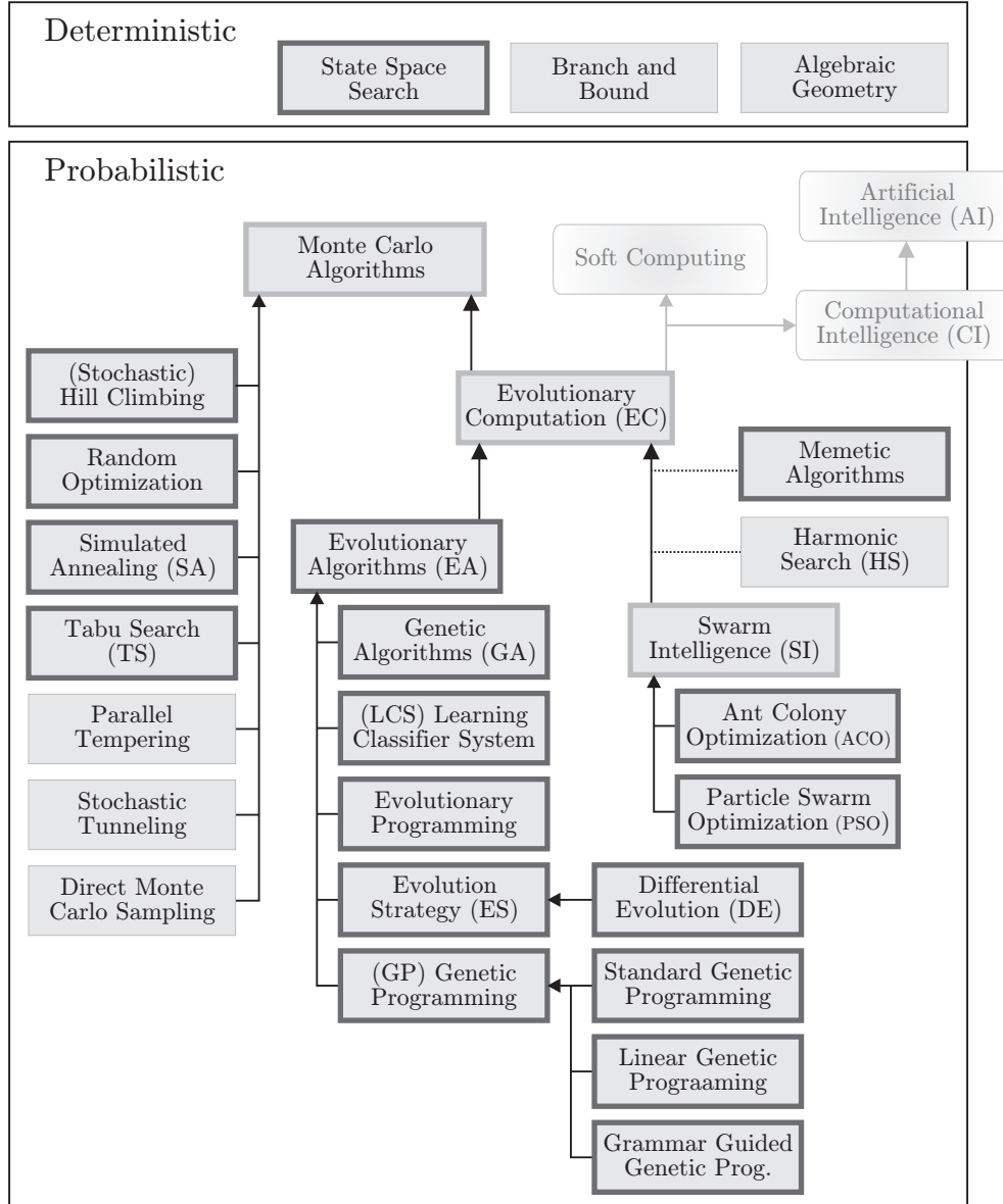
Fig. 1.1: The taxonomy of global optimization algorithms.
