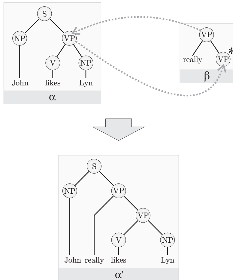
Fig. 29.17: An example for the adjunction operation.
