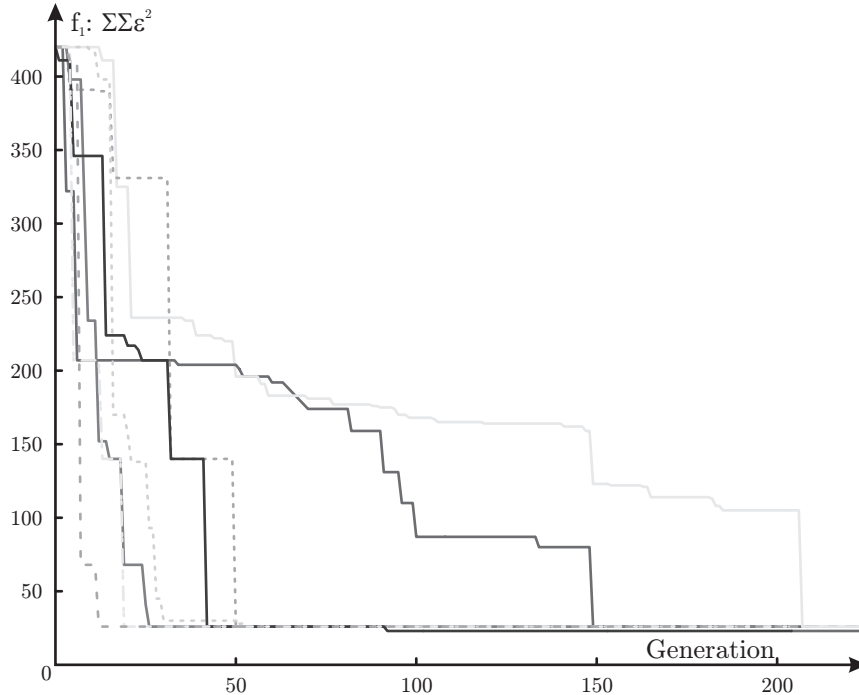
Fig. 23.19: The evolutionary progress of the static average protocol.
