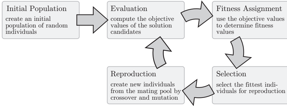
Fig. 2.1: The basic cycle of evolutionary algorithms.
