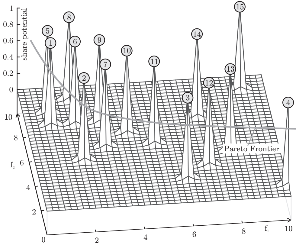
Fig. 2.5: The sharing potential in the Variety Preserving Ranking example
