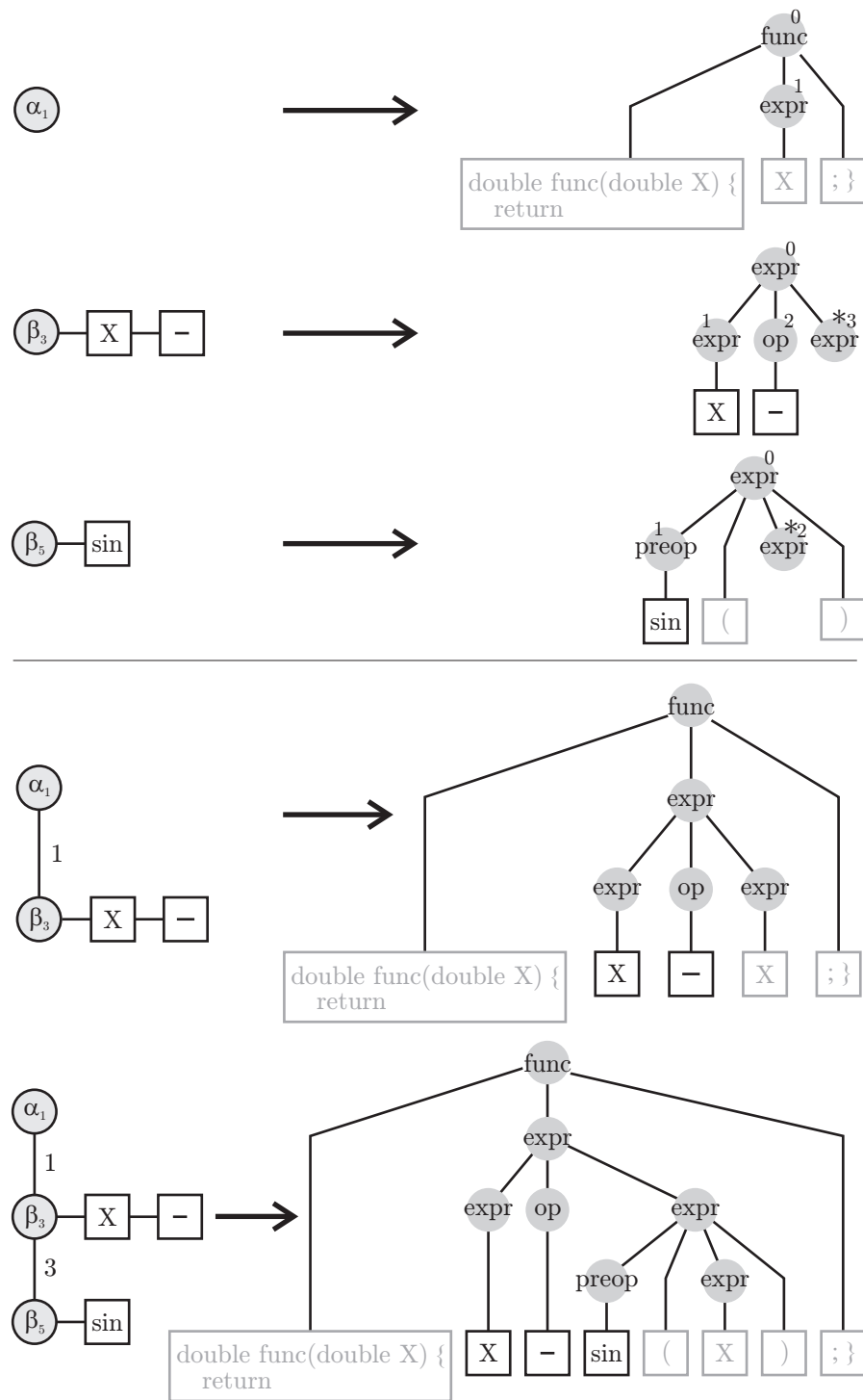
Fig. 4.20: One example genotype-phenotype mapping in TAG3P.
