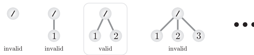
Fig. 4.16: Example for valid and invalid trees in symbolic regression.
