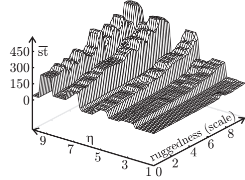
Fig. 20.13.2: The experimentally obtained results.
