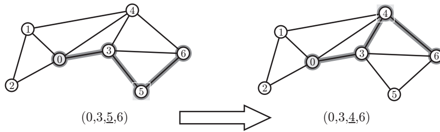
Fig. 23.6.1: The path mutation operator.
