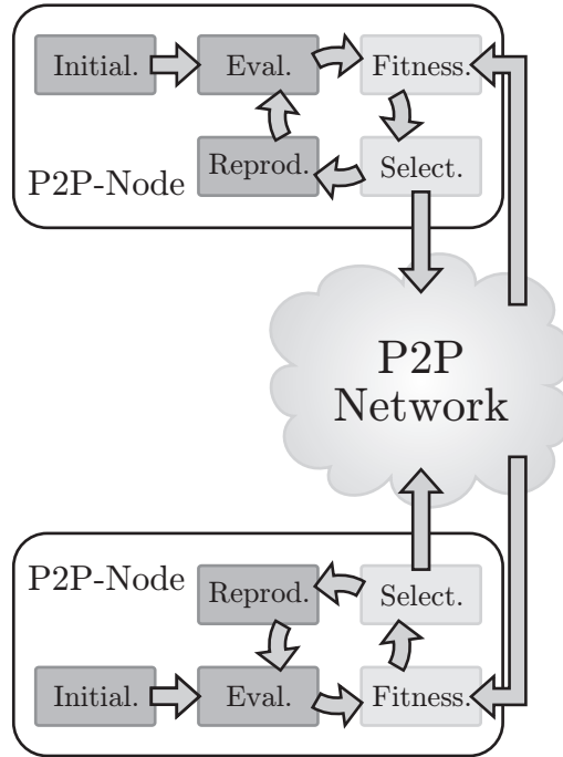
Fig. 17.5: An evolutionary algorithm distributed in a P2P network.
