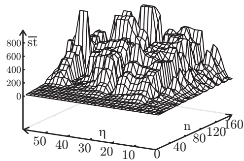
Fig. 20.10.1: Epistasis \eta and problem length n .
