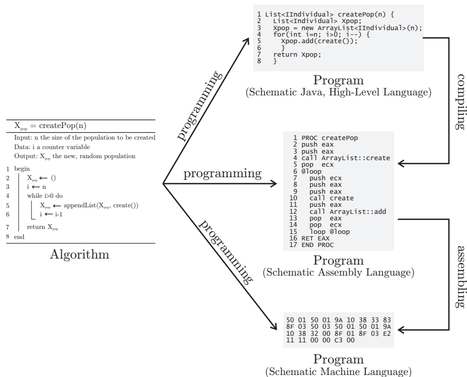
Fig. 29.1: The relation between algorithms and programs.
