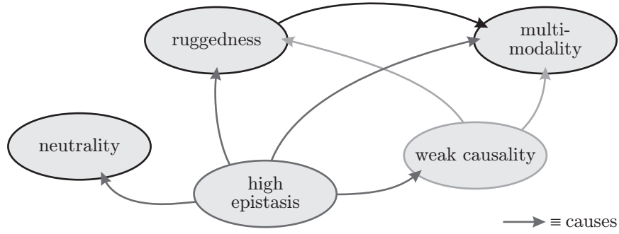
Fig. 1.22: The influence of epistasis on the fitness landscape.
