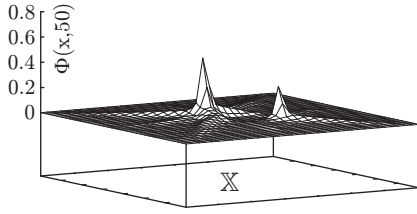
Fig. 1.18.5: \Phi(x, 50)
