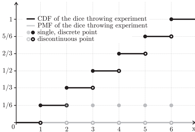
Fig. 27.17: The PMF and CMF of the dice throw
