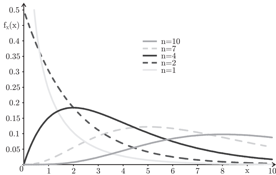
Fig. 27.13: The PDFs of some \chi^2 distributions
