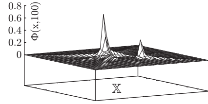
Fig. 1.18.6: \Phi(x, 100)
