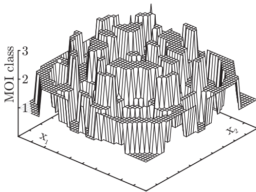
Fig. 1.11.2: The Method of Inequalities class division.
