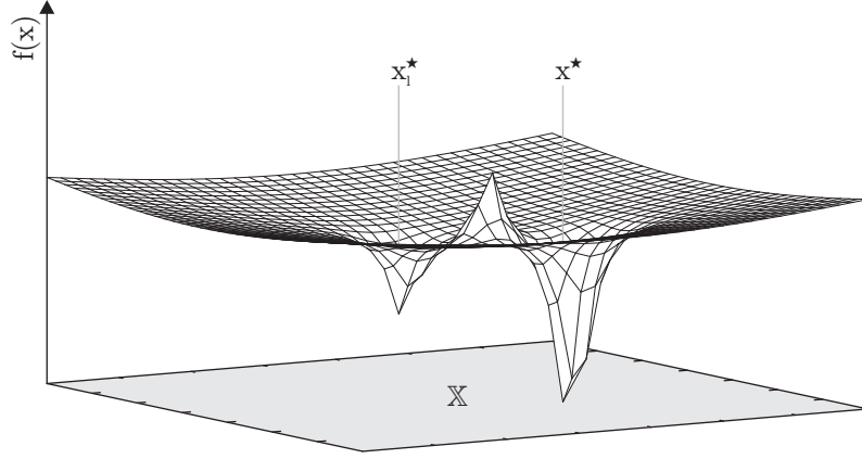
Fig. 1.16: An example optimization problem.
