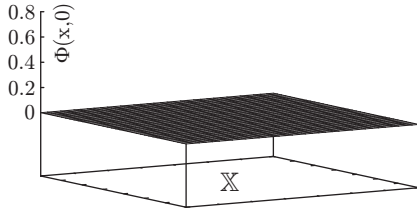
Fig. 1.18.1: \Phi(x, 1)
