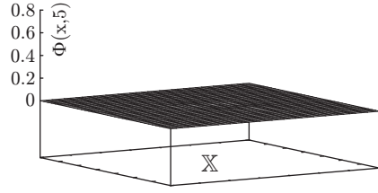
Fig. 1.17.3: \Phi(x, 5)
