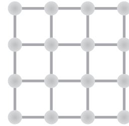
Fig. 29.3.6: grid
