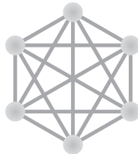
Fig. 29.3.7: fully connected
