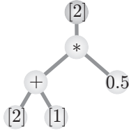
Fig. 23.18.1: distributed average
