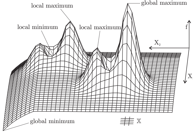
Fig. 1.2: Global and local optima of a two-dimensional function.
