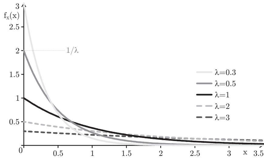
Fig. 27.11: The PDFs of some exponential distributions
