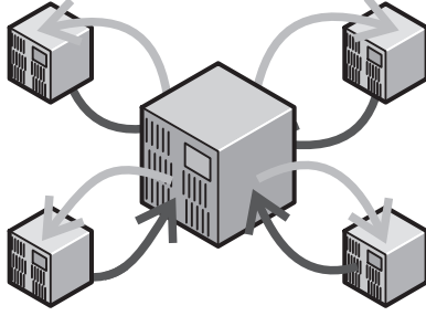
Fig. 23.11.1: reactive aggregation
