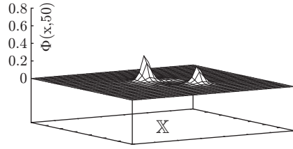
Fig. 1.17.5: \Phi(x, 50)
