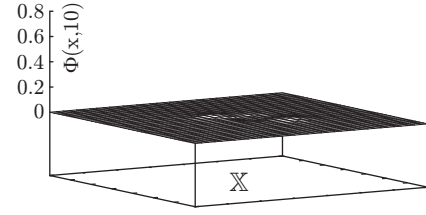
Fig. 1.17.4: \Phi(x, 10)
