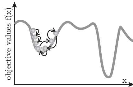
Fig. 1.19.2: Example 2: Minimization
