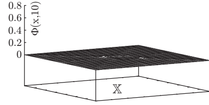
Fig. 1.18.4: \Phi(x, 10)
