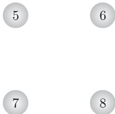
Fig. 23.13.1: initial state
