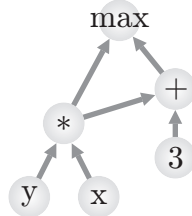
Fig. 4.23.2: graph structure
