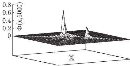
Fig. 1.18.11: \Phi(x, 6000)
