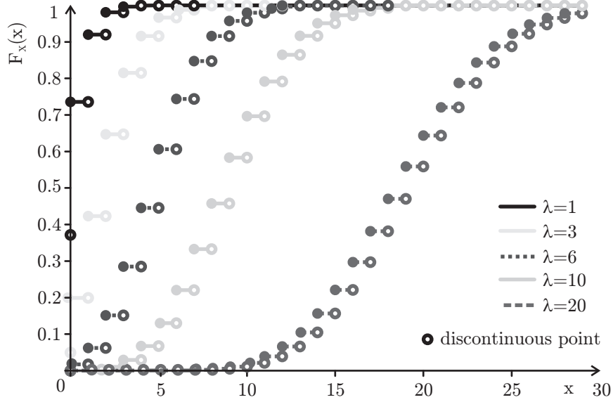
Fig. 27.4: The CDFs of some Poisson distributions
