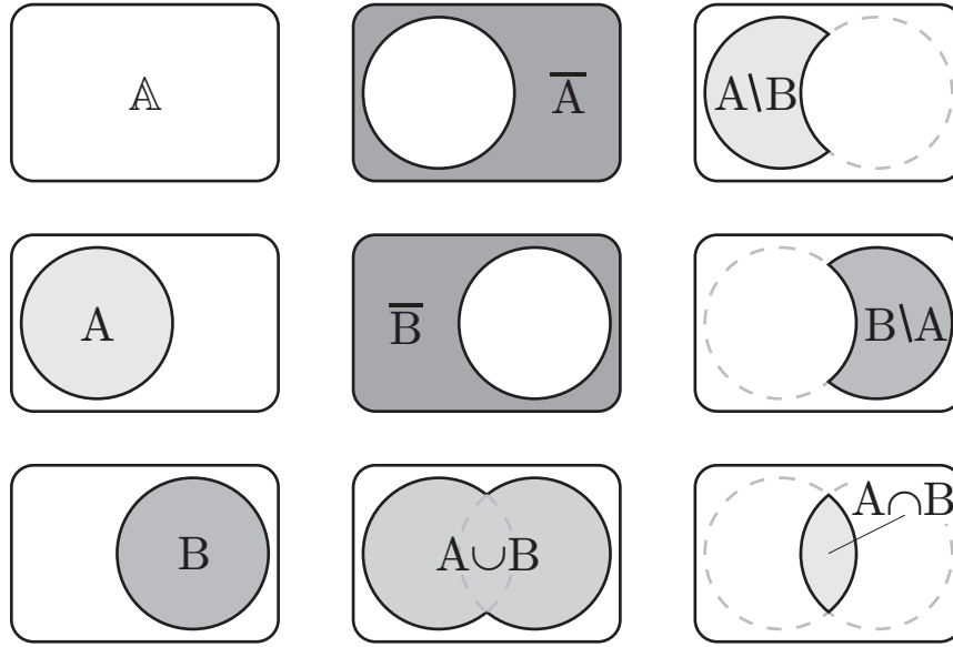
Fig. 26.1: Set operations performed on sets A and B inside a set \mathbb{A}
