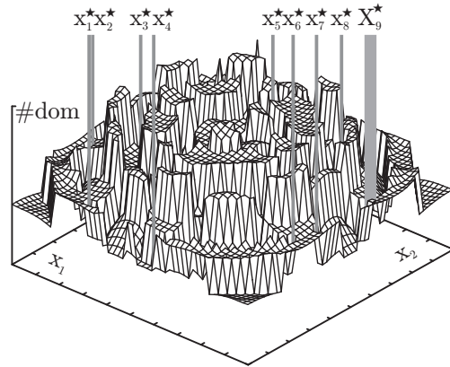
Fig. 1.11.3: The Method of Inequalities ranking.
