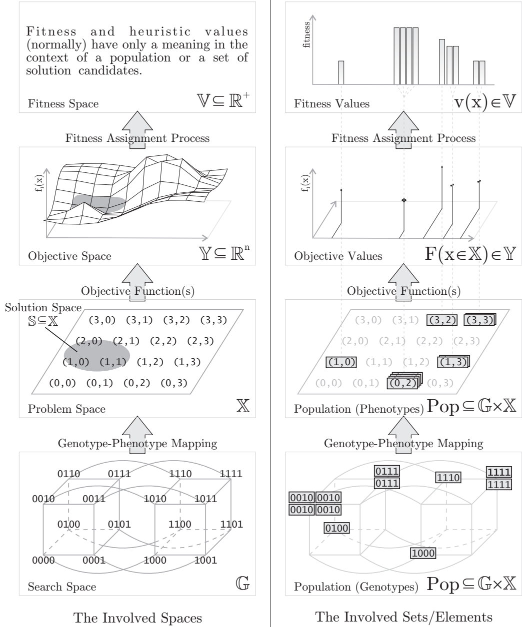
Fig. 1.13: Spaces, Sets, and Elements involved in an optimization process.
