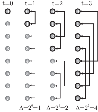
Fig. 23.14.1: pair-based
