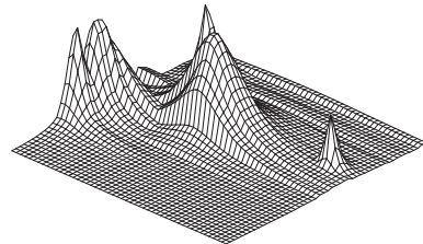
Fig. 20.1.8: t = 13
