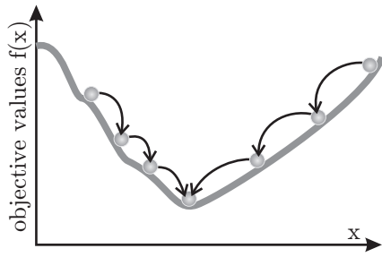
Fig. 1.20.1: Best case
