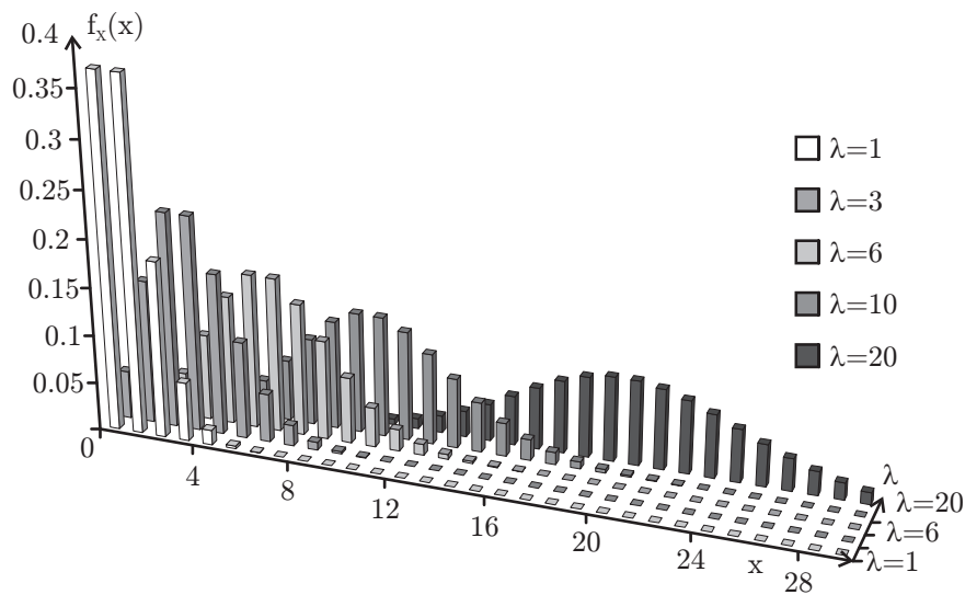
Fig. 27.3: The PMFs of some Poisson distributions
