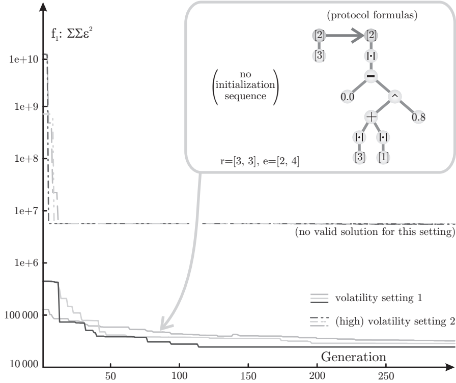
Fig. 23.25: The evolutionary progress and one grown solution of the dynamic root-of-average protocol.
