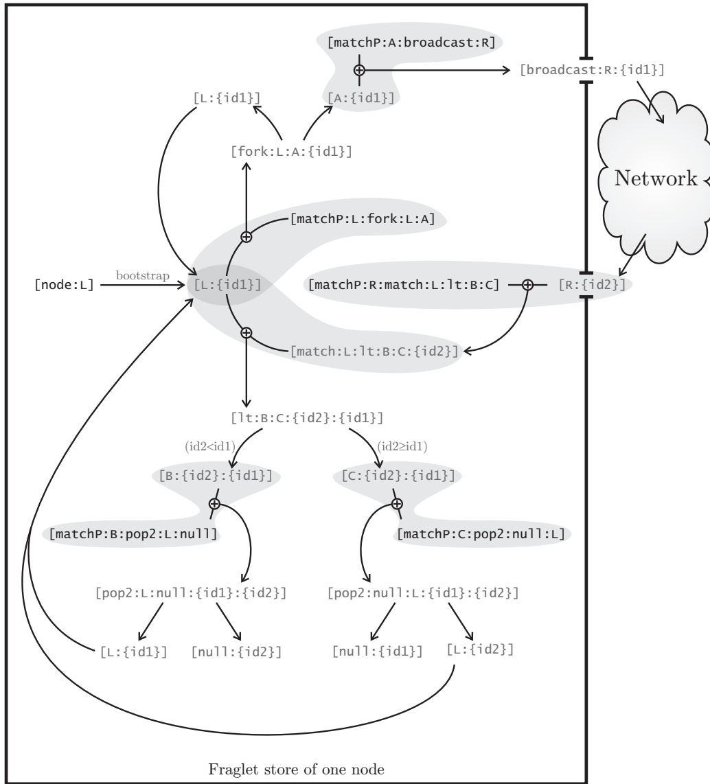
Fig. 4.32: A Fraglet-based election algorithm
