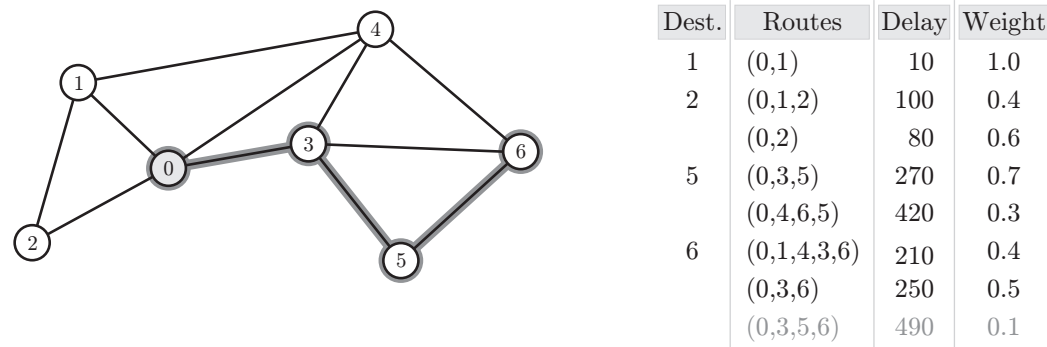
Fig. 23.5: The table with the most frequently used routes of node 0.
