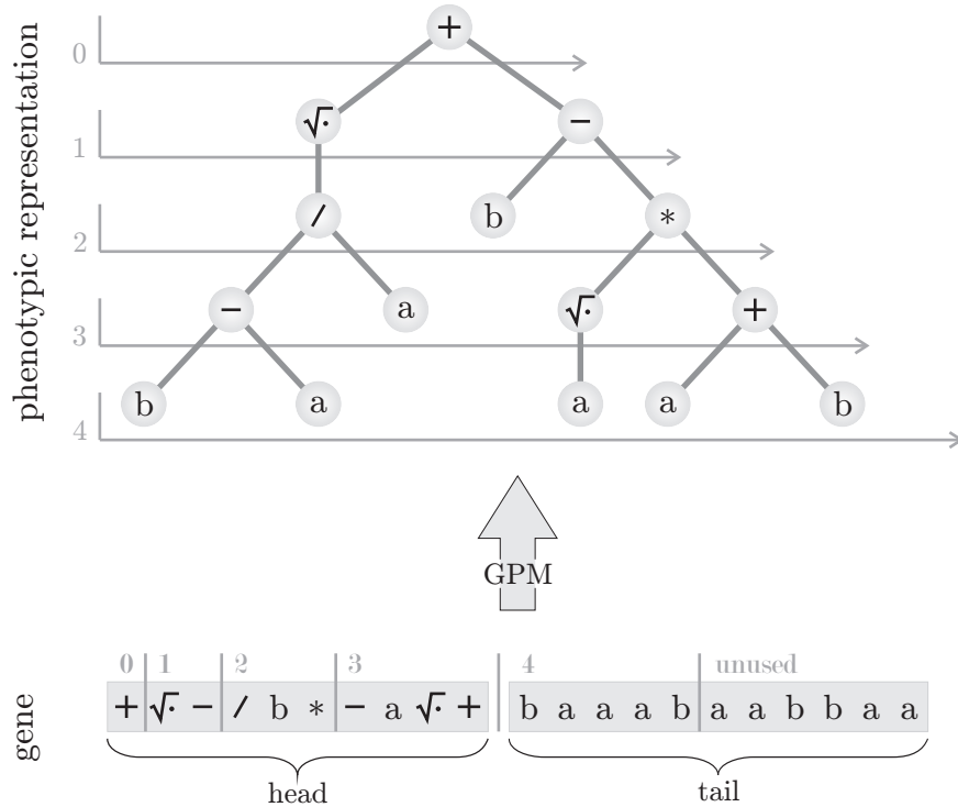
Fig. 4.14: A GPM example for Gene Expression Programming.
