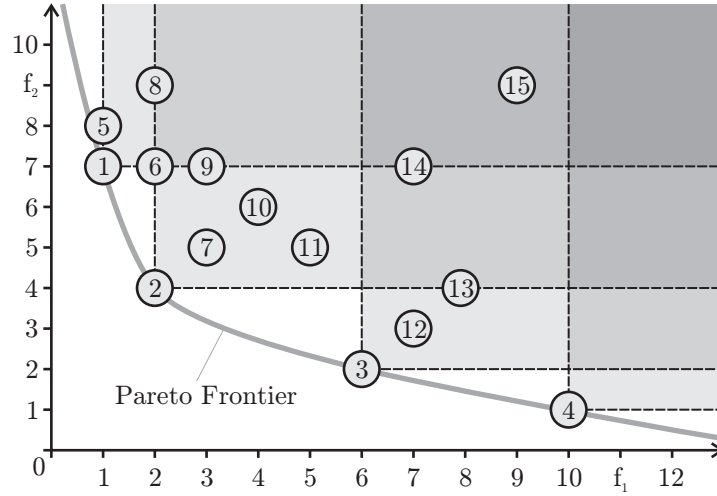
Fig. 2.4: An example scenario for Pareto ranking.
