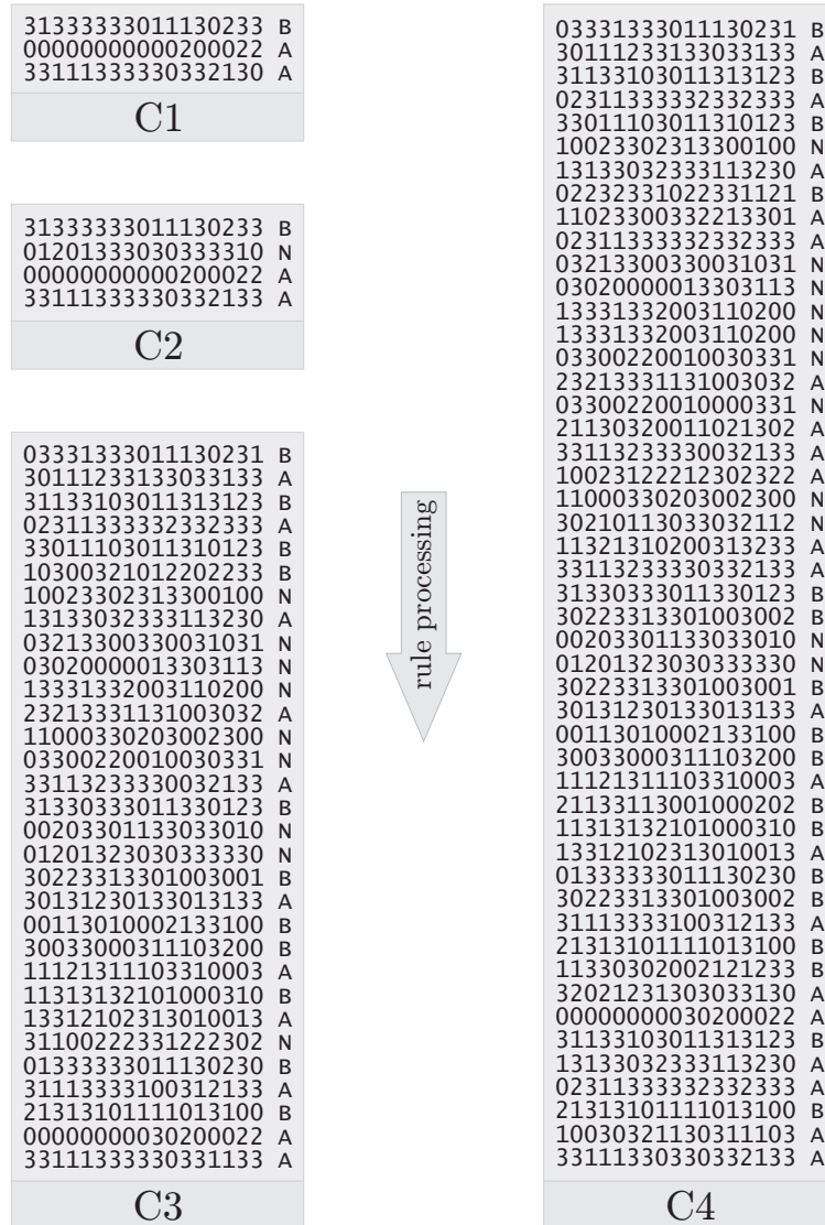
Fig. 21.6: Some Pareto-optimal individuals among the evolved classifier systems.
