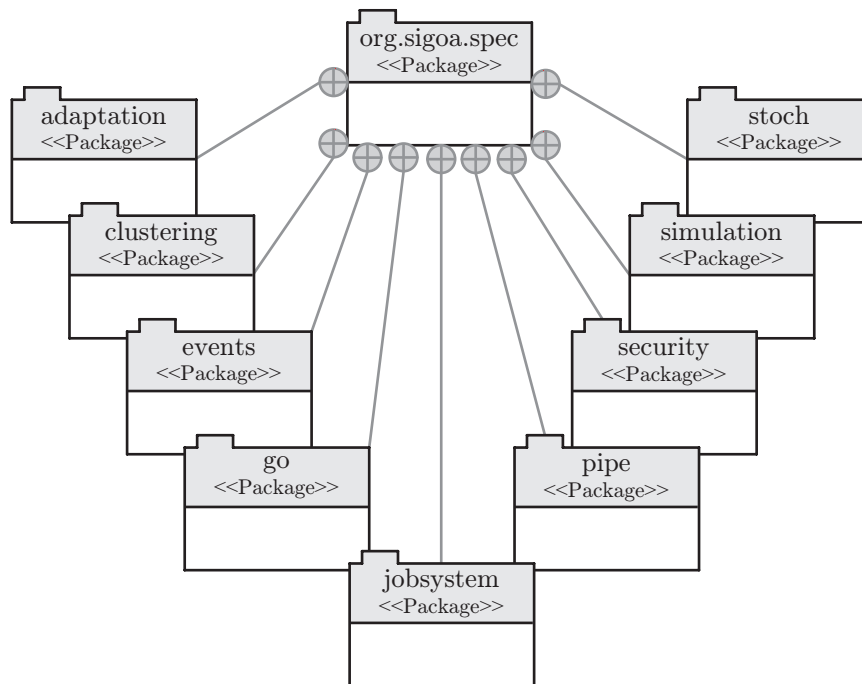
Fig. 24.2: The subsystem specification of the optimization framework.
