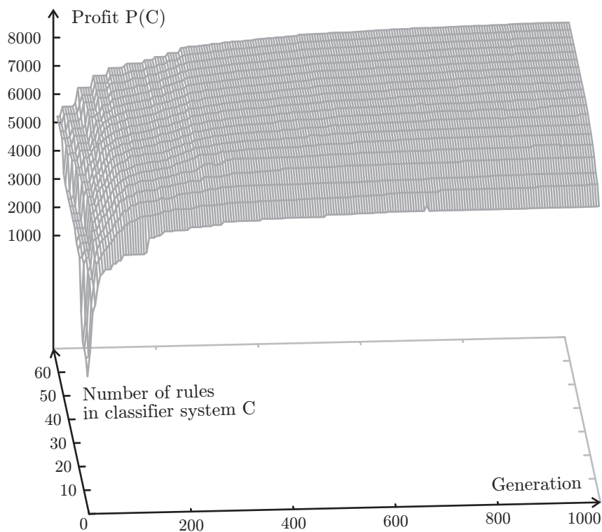
Fig. 21.5: The course of the classifier system evolution.
