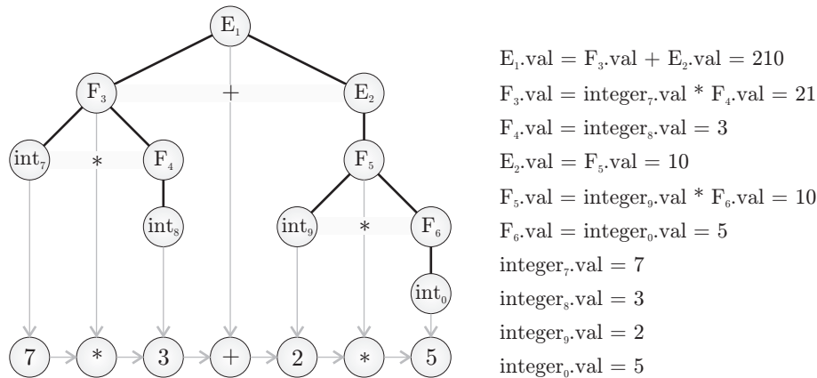
Fig. 29.13: An instantiation of the grammar from Listing 29.7.
