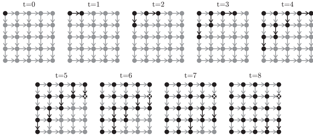
Fig. 23.7: The application of Listing 23.1 to a 5 \times 5 grid.
