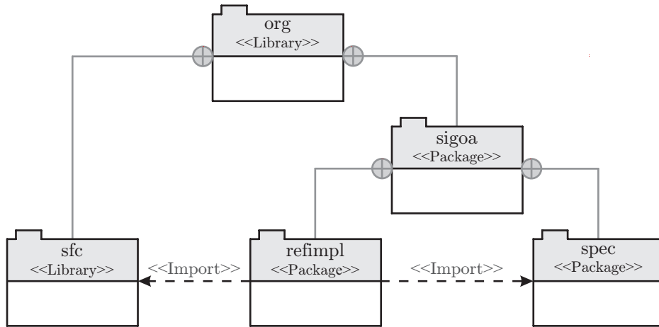
Fig. 24.1: The top-level packages of the Sigoa optimization system.
