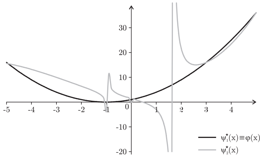
Fig. 22.2: \varphi(x) , the evolved \psi_1^*(x) \equiv \varphi(x) , and \psi_2^*(x) .
