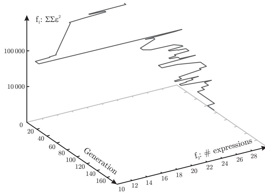
Fig. 23.26: The relation of f_1 and f_2 in the dynamic root-of-average protocol.
