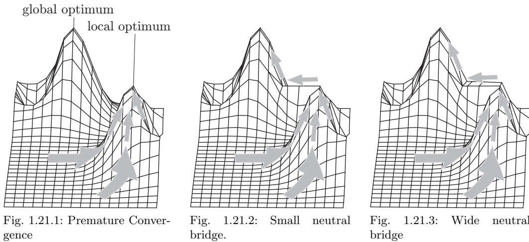
Fig. 1.21: Possible positive influence of neutrality.
