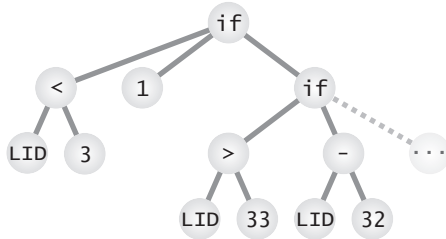
Fig. 23.3.1: The RFS approach.
