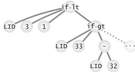
Fig. 23.3.2: The decision tree method (DT).
