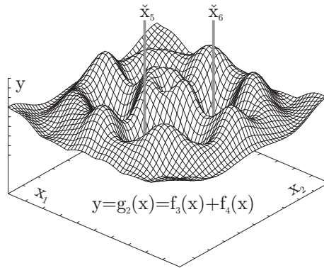
Fig. 1.6: Optimization using the weighted sum approach (second example).
