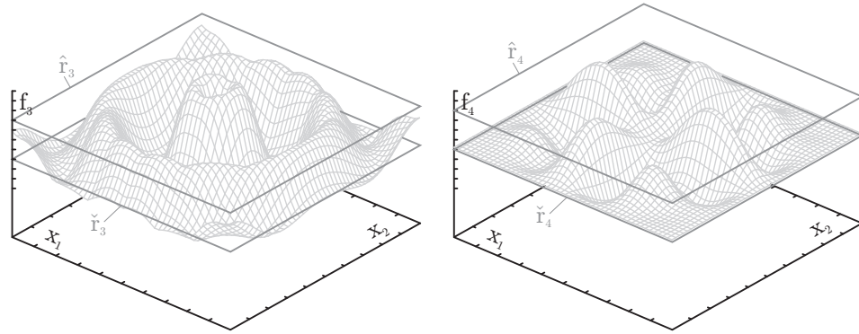
Fig. 1.11.1: The ranges applied to f_3 and f_4 .
