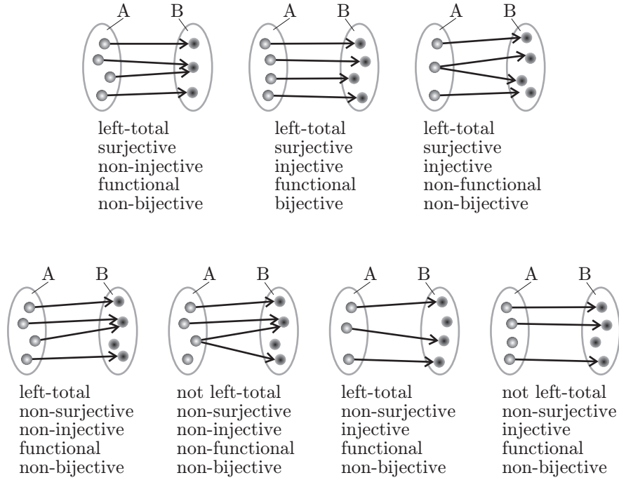
Fig. 26.2: Properties of a binary relation R with domain A and codomain B .
