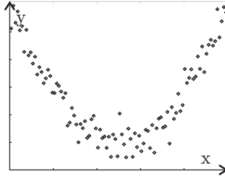
Fig. 1.24.2: The measurement/training data.
