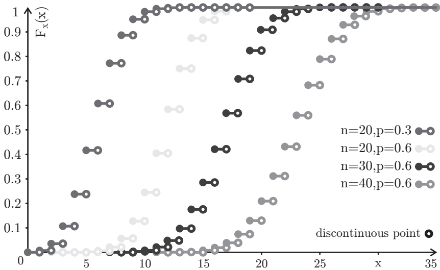
Fig. 27.6: The CDFs of some binomial distributions
