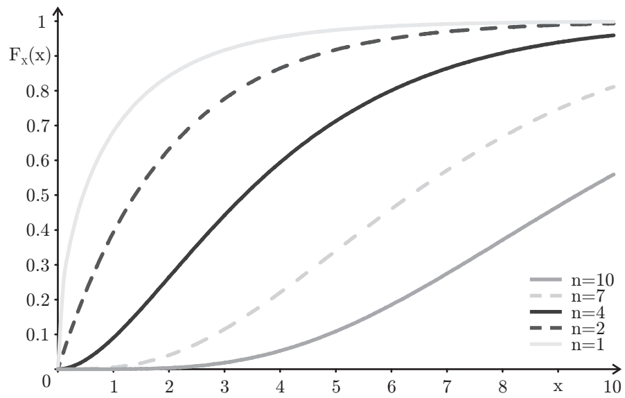
Fig. 27.14: The CDFs of some \chi^2 distributions
