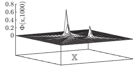
Fig. 1.18.8: \Phi(x, 1000)
