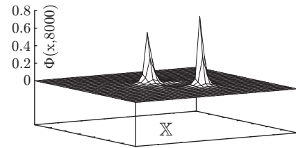
Fig. 1.17.12: \Phi(x, 8000)
