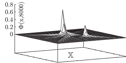
Fig. 1.18.12: \Phi(x, 8000)
