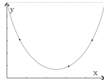
Fig. 1.25.3: The oversimplified result.
