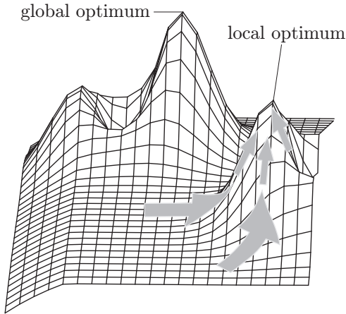
Fig. 1.19.1: Example 1: Maximization
