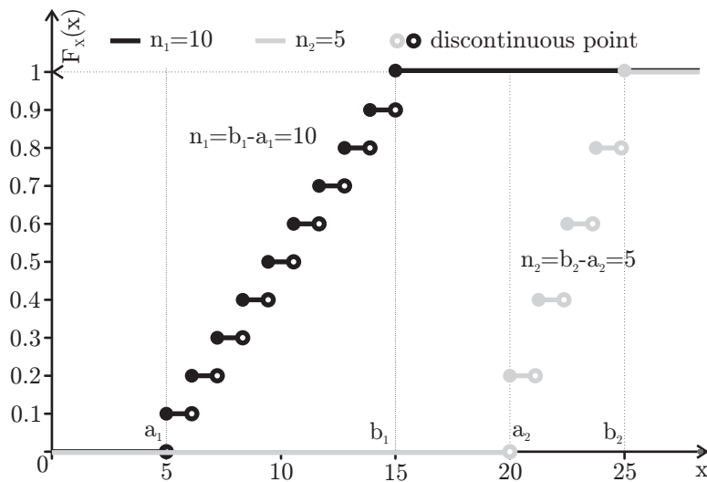
Fig. 27.2: The CDFs of some discrete uniform distributions
