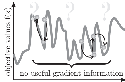
Fig. 1.20.4: Rugged
