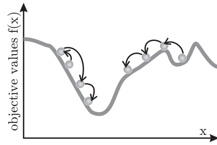
Fig. 1.20.2: Low Variation
