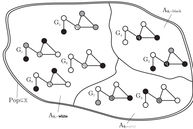
Fig. 1.28: An graph coloring-based example for properties and formae.
