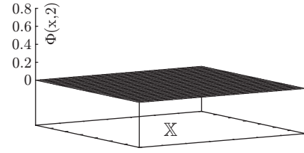
Fig. 1.18.2: \Phi(x, 2)
