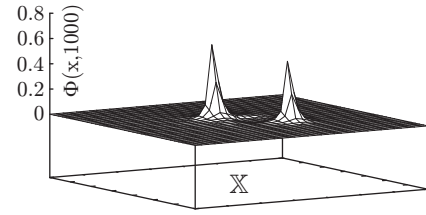
Fig. 1.17.8: \Phi(x, 1000)
