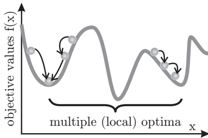
Fig. 1.20.3: Multimodal
