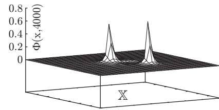
Fig. 1.17.10: \Phi(x, 4000)
