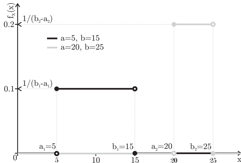
Fig. 27.7: The PDFs of some continuous uniform distributions
