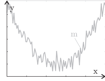
Fig. 1.24.3: The overfitted result.
