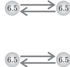
Fig. 23.13.3: after step 2
