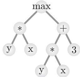
Fig. 4.23.1: tree structure
