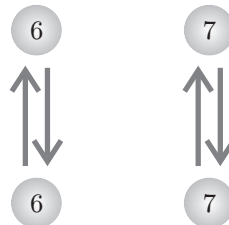
Fig. 23.13.2: after step 1
