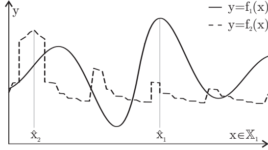
Fig. 1.3: Two functions f_1 and f_2 with different maxima \hat{\mathbf{x}}_1 and \hat{\mathbf{x}}_2 .
