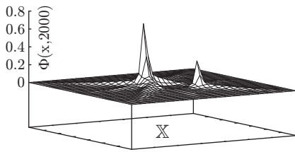
Fig. 1.18.9: \Phi(x, 2000)
