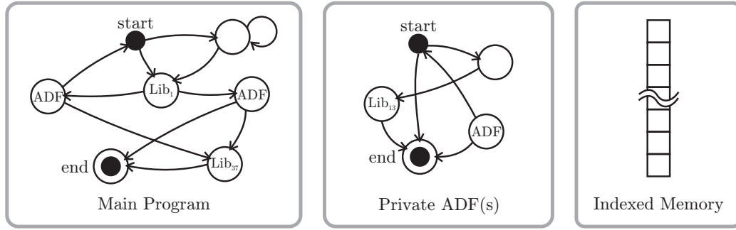
Fig. 4.22: The general structure of a Parallel Algorithm Discovery and Orchestration program.
