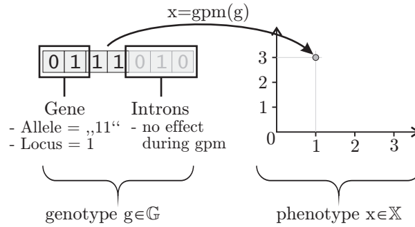
Fig. 3.2: A four bit string genome \mathbb{G} and a fictitious phenotype \mathbb{X} .
