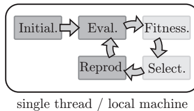
Fig. 17.2: A sequentially proceeding evolutionary algorithm.
