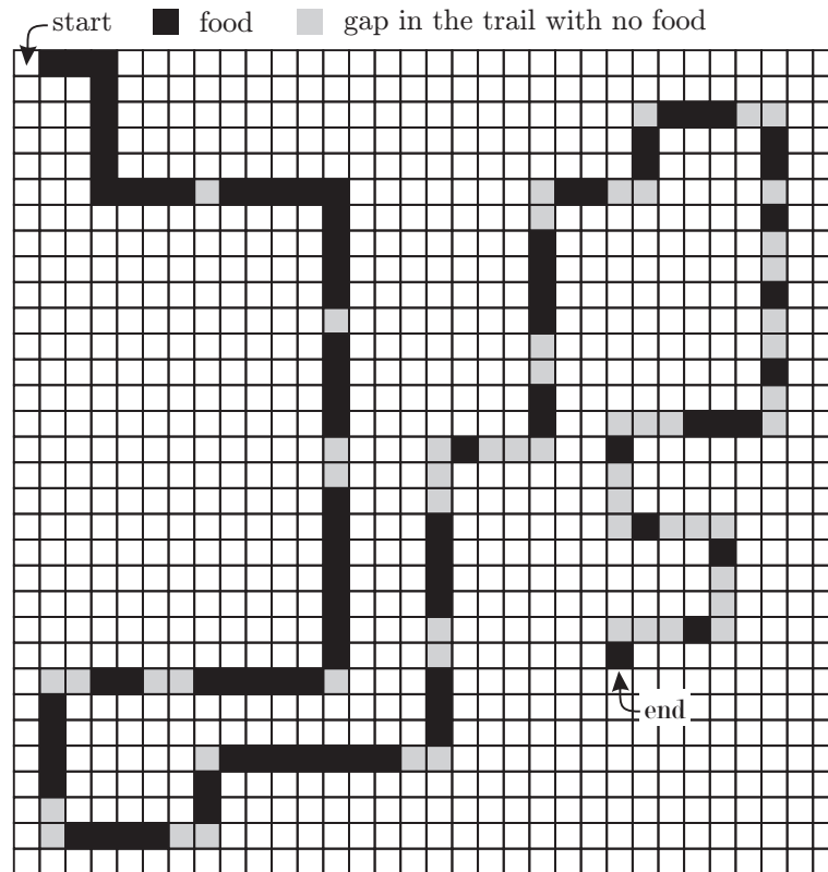
Fig. 20.14: The Santa Fee Trail in the Artificial Ant Problem [65].
