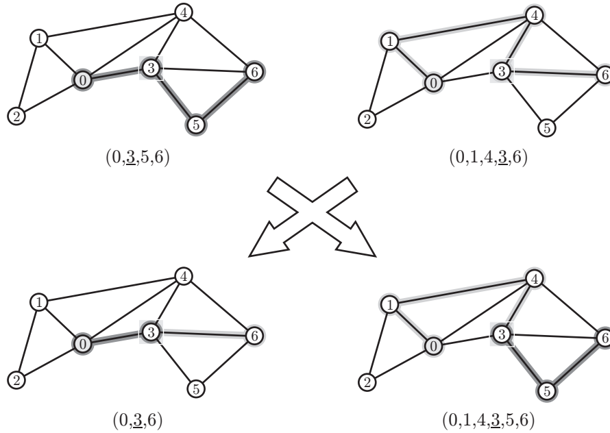
Fig. 23.6.2: The path mutation operator.
