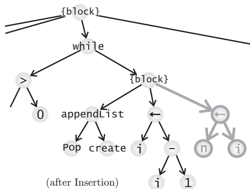
Fig. 4.21.2: Inserting in a tree representation.
