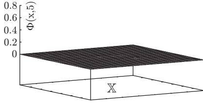
Fig. 1.18.3: \Phi(x, 5)
