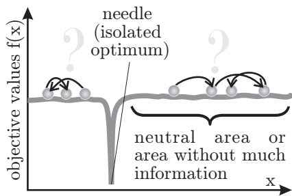
Fig. 1.20.7: Needle-In-A-Haystack
