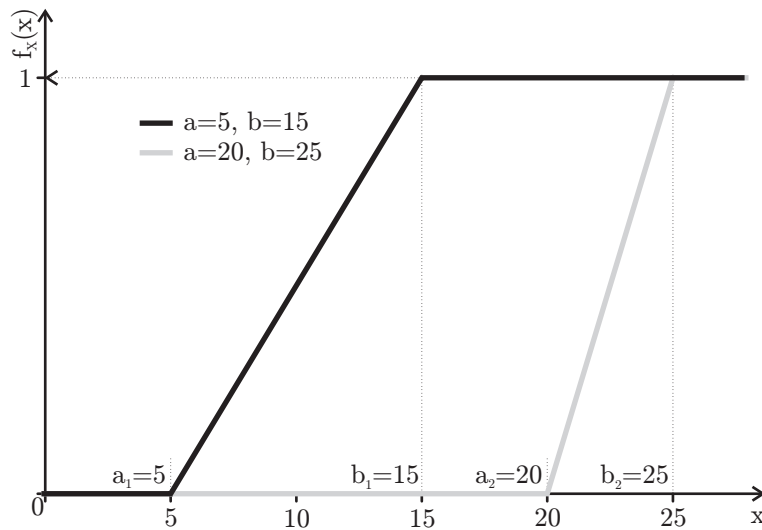
Fig. 27.8: The CDFs of some continuous uniform distributions
