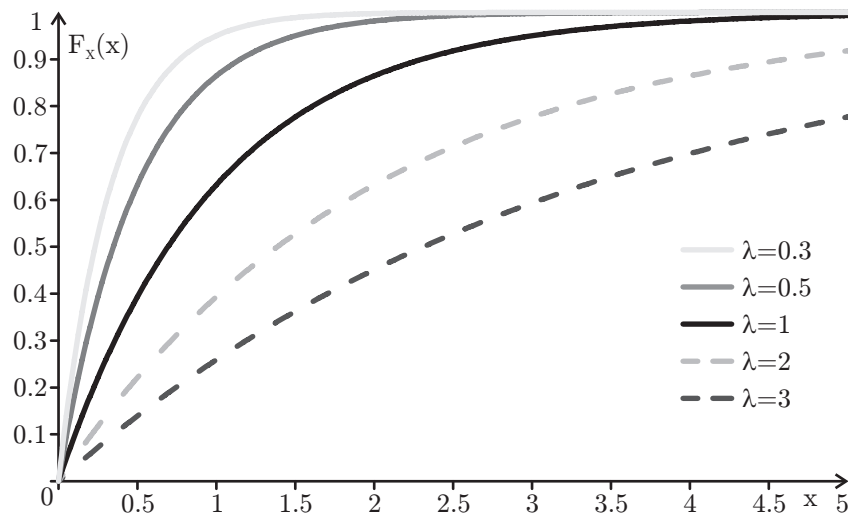
Fig. 27.12: The CDFs of some exponential distributions
