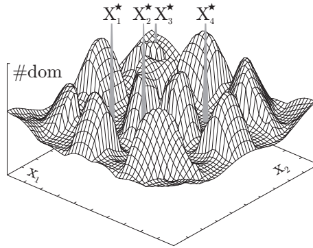
Fig. 1.9: Optimization using the Pareto Frontier approach (second example).
