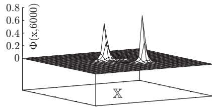
Fig. 1.17.11: \Phi(x, 6000)
