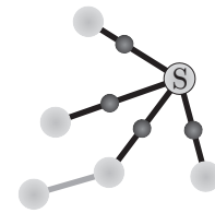
Fig. 29.11.3: Broadcast
