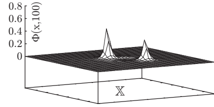
Fig. 1.17.6: \Phi(x, 100)
