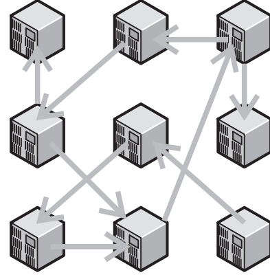
Fig. 23.11.2: proactive aggregation
