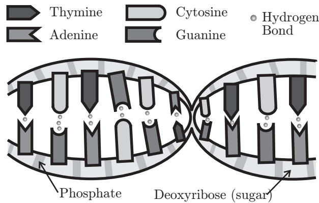
Fig. 1.14: A sketch of a part of a DNA molecule.
