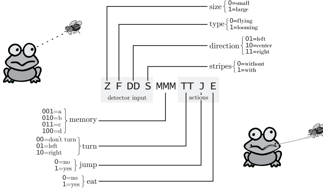
Fig. 7.2: One possible encoding of messages for a frog classifier system
