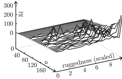
Fig. 20.9.2: Scaled ruggedness \bar{st} plot.
